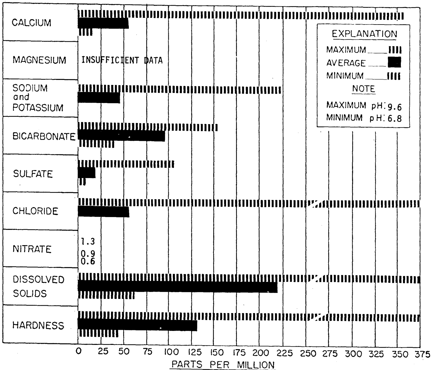
MAXIMUM, AVERAGE, and MINIMUM concentrations of dissolved constituents, Green River at Munfordville
