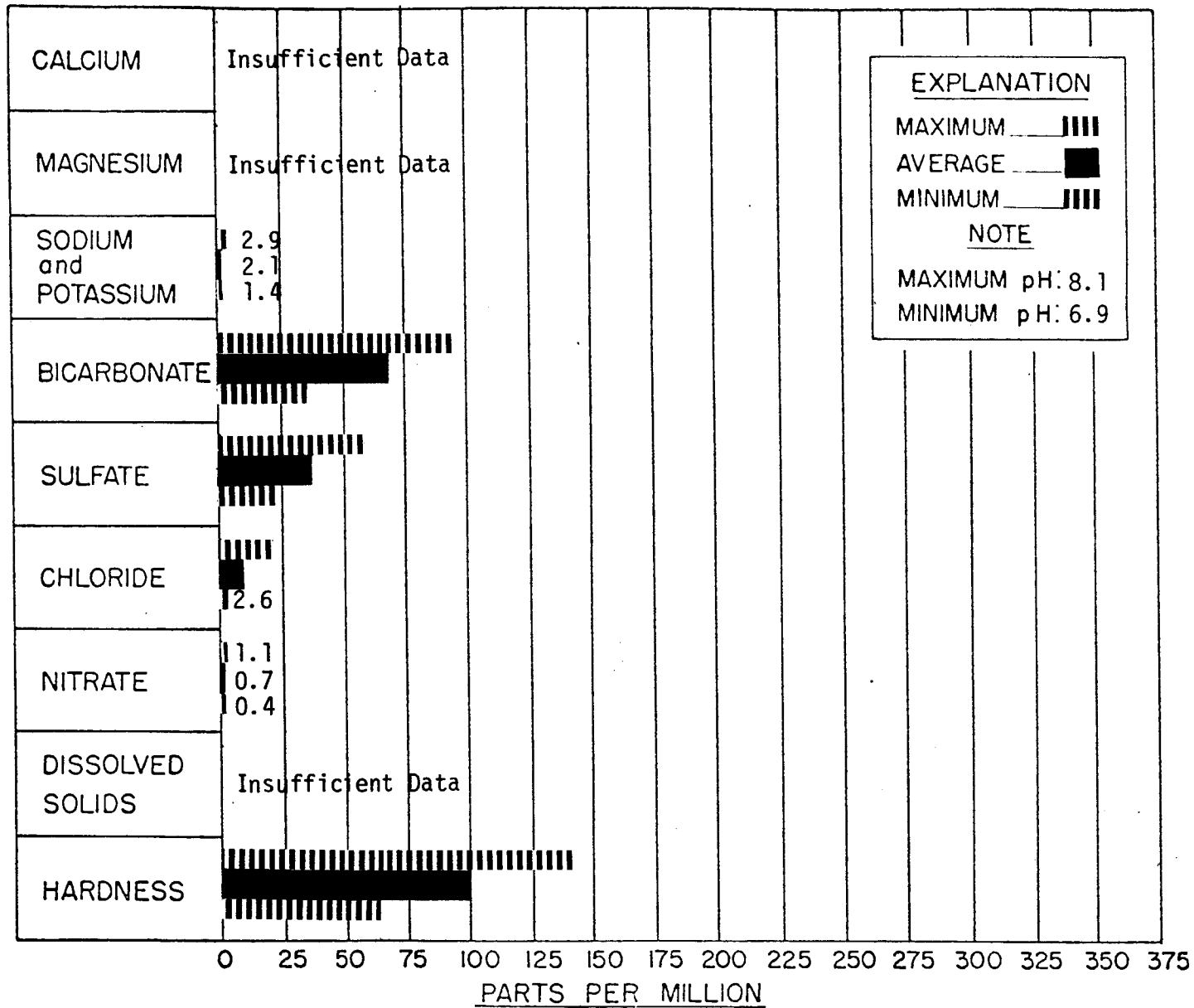
MAXIMUM, AVERAGE, and MINIMUM concentrations of dissolved constituents, Kentucky River, Lock 4 at Frankfort Period of Record 1-73 to 11-74
