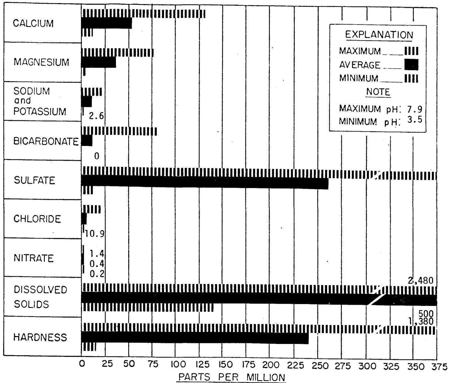
MAXIMUM, AVERAGE, and MINIMUM concentrations of dissolved constituents, Trade Water River at Olney Period of Record 2-59 to 9-73
