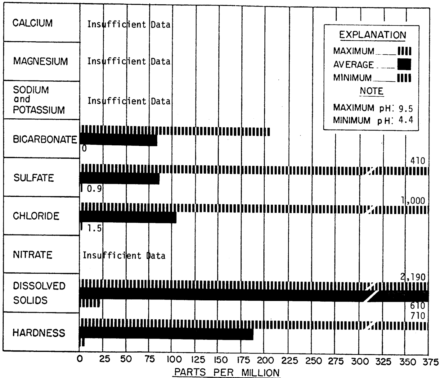
MAXIMUM, AVERAGE, and MINIMUM concentrations of dissolved constituents, North Fork Ky. River at Hazard Period of Record 1-73 to 6-74
