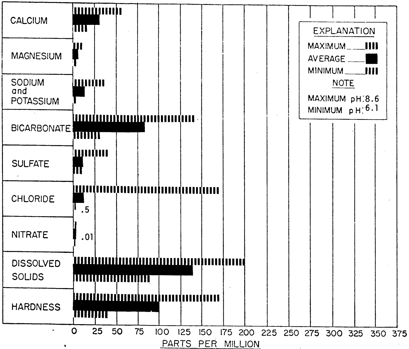
MAXIMUM, AVERAGE, and MINIMUM concentrations of dissolved constituents, Licking River at McKinneysburg. Period of Record 10-59 to 10-73
