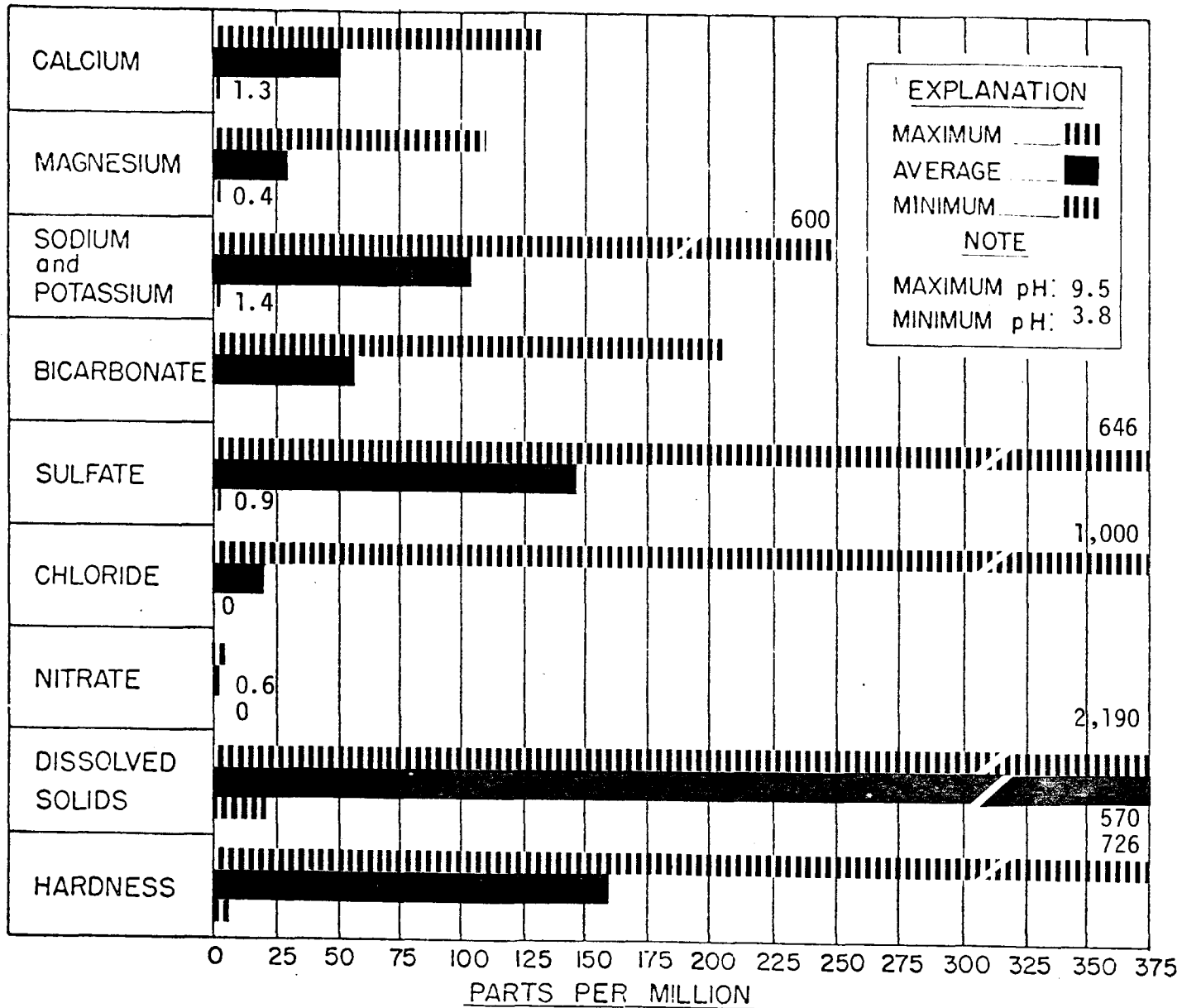
MAXIMUM, AVERAGE, and MINIMUM concentrations of dissolved constituents, N. Fork Kentucky R. at Hazard Period of Record 10-62 to 6-74
