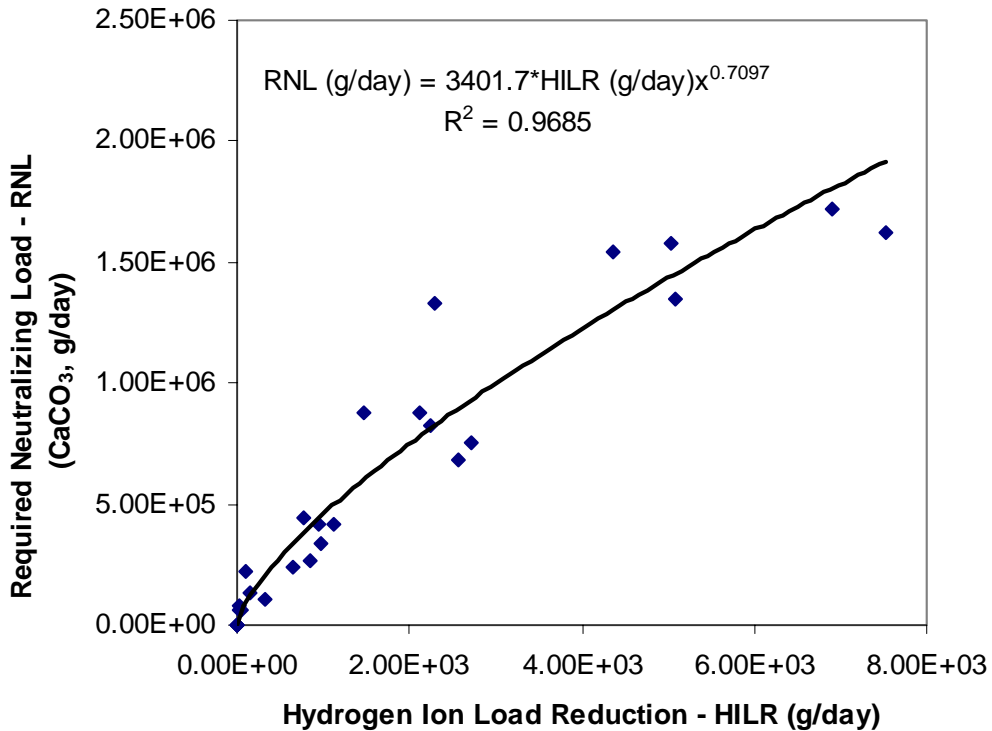
Figure 10. CaCO 3 Loading vs. Required Hydrogen Ion Reduction
