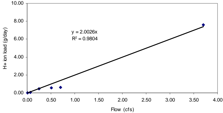
Figure 9. Relation Between Flow and Ion Load for Site 6
