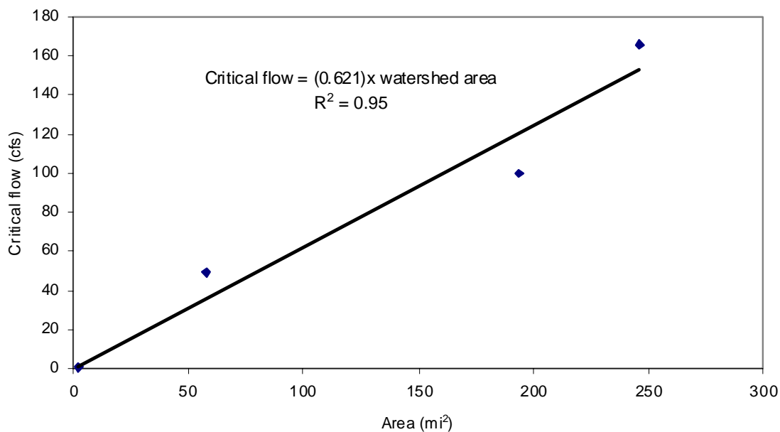
Figure 5. Relation Between Drainage Area and the Critical TMDL Flow
