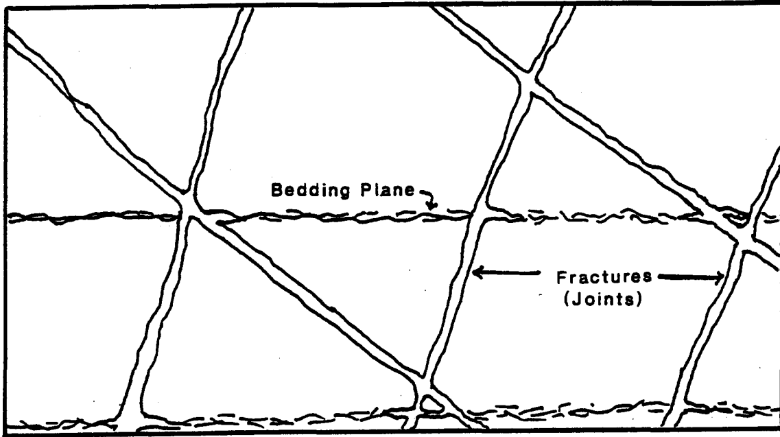
Figure 6. Interconnected Fractures and Bedding Planes in Limestones. Such fractures provide secondary permeability to the rock mass, allowing groundwater to flow through them (modified after Smith and others, 1982).
