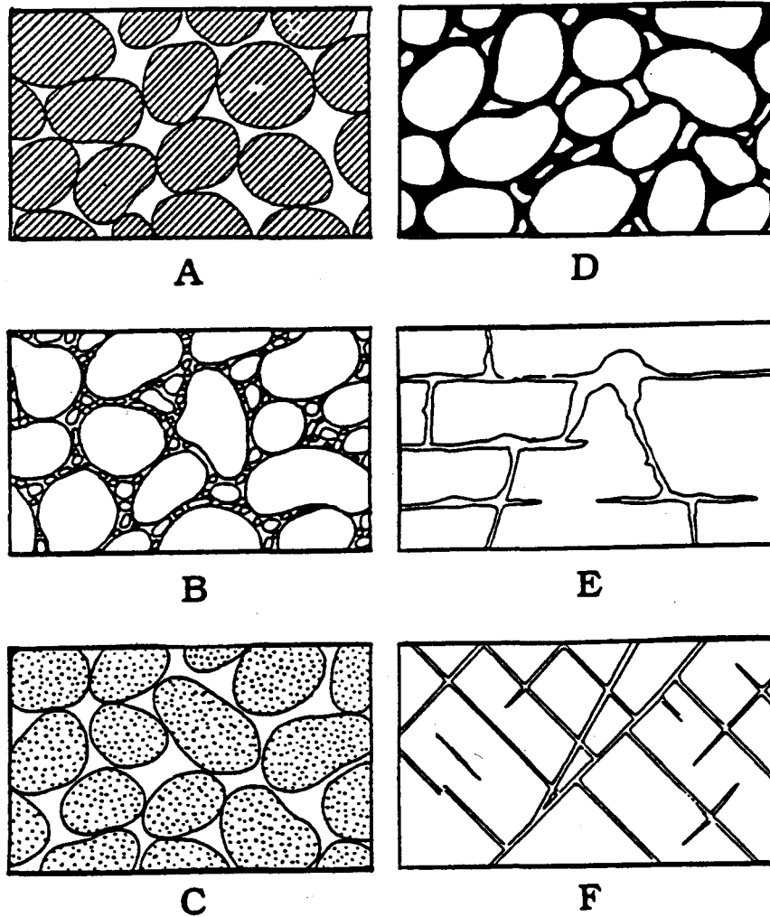
Figure 4. Types of Pore Spaces and the Relationship of Rock Texture to Porosity. (A) Well-sorted sediments having high primary porosity; (B) poorly sorted sediments having low primary porosity; (C) well-sorted, porous sedimentary grains with open pore spaces; (D) well-sorted sedimentary deposit having diminished porosity due to deposition of cement in pore spaces; (E) rock having secondary porosity due to solution; (F) rock having secondary porosity due to fractures (modified after O. E. Meinzer, 1923).
