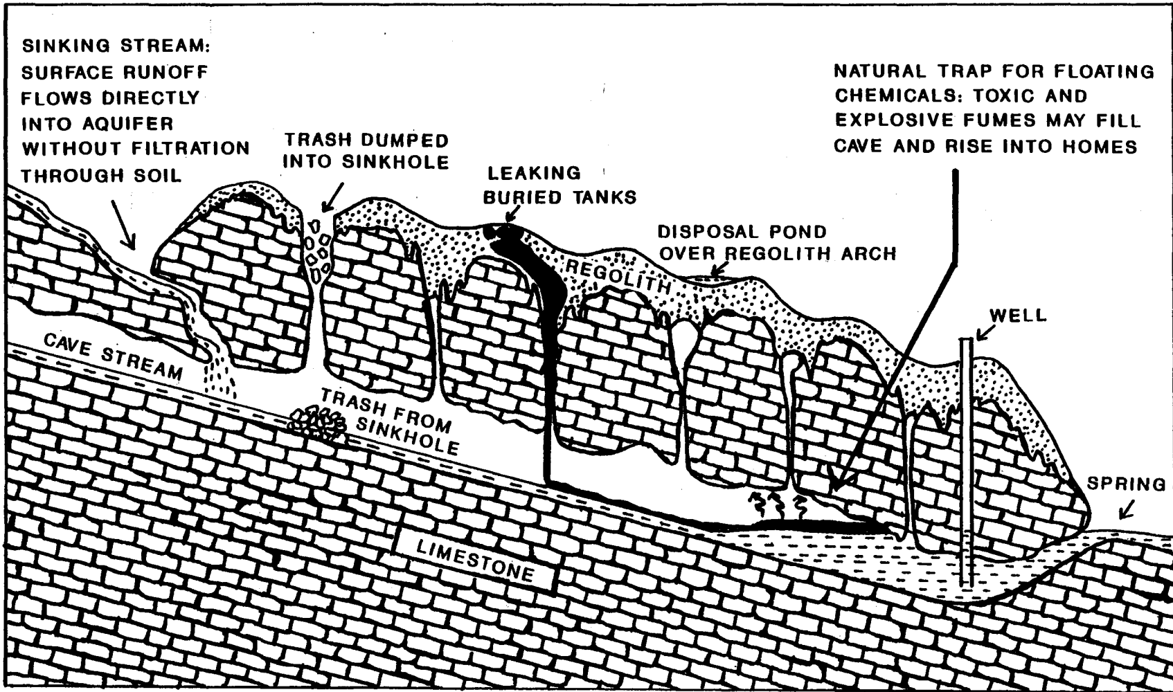
Figure 11. Sources of Contamination of Karst Groundwater (Crawford, 1988).
