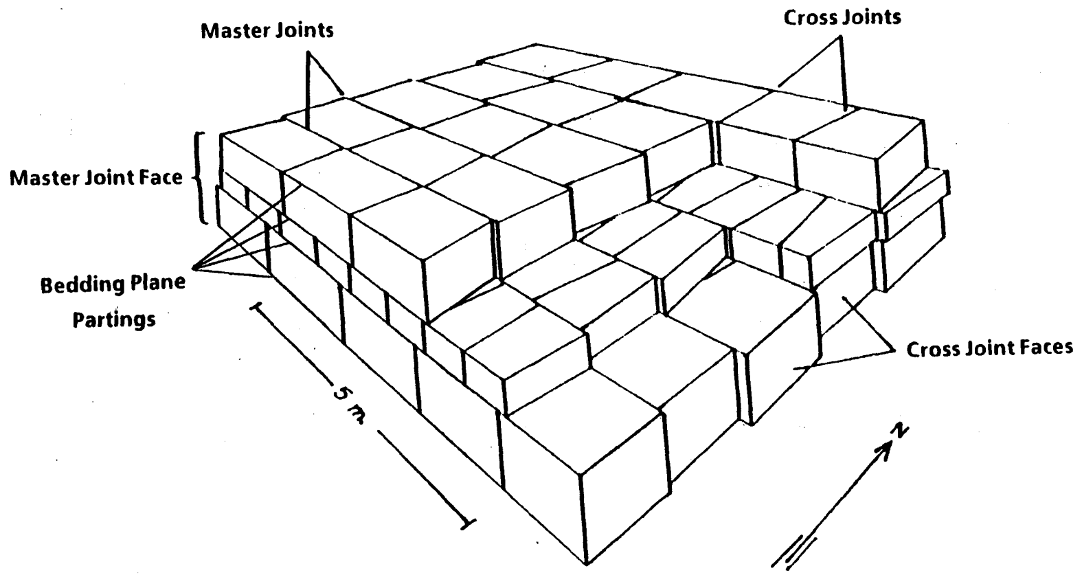
Figure 5. Block Diagram Illustrating Common Fracture Patterns in Limestone Bedrock (modified after Powell, 1977).
