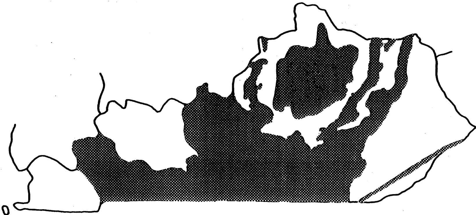
Figure 2. Areas of Potential Karst Groundwater Flow in Kentucky. Patterned areas indicate potential karst groundwater flow.
