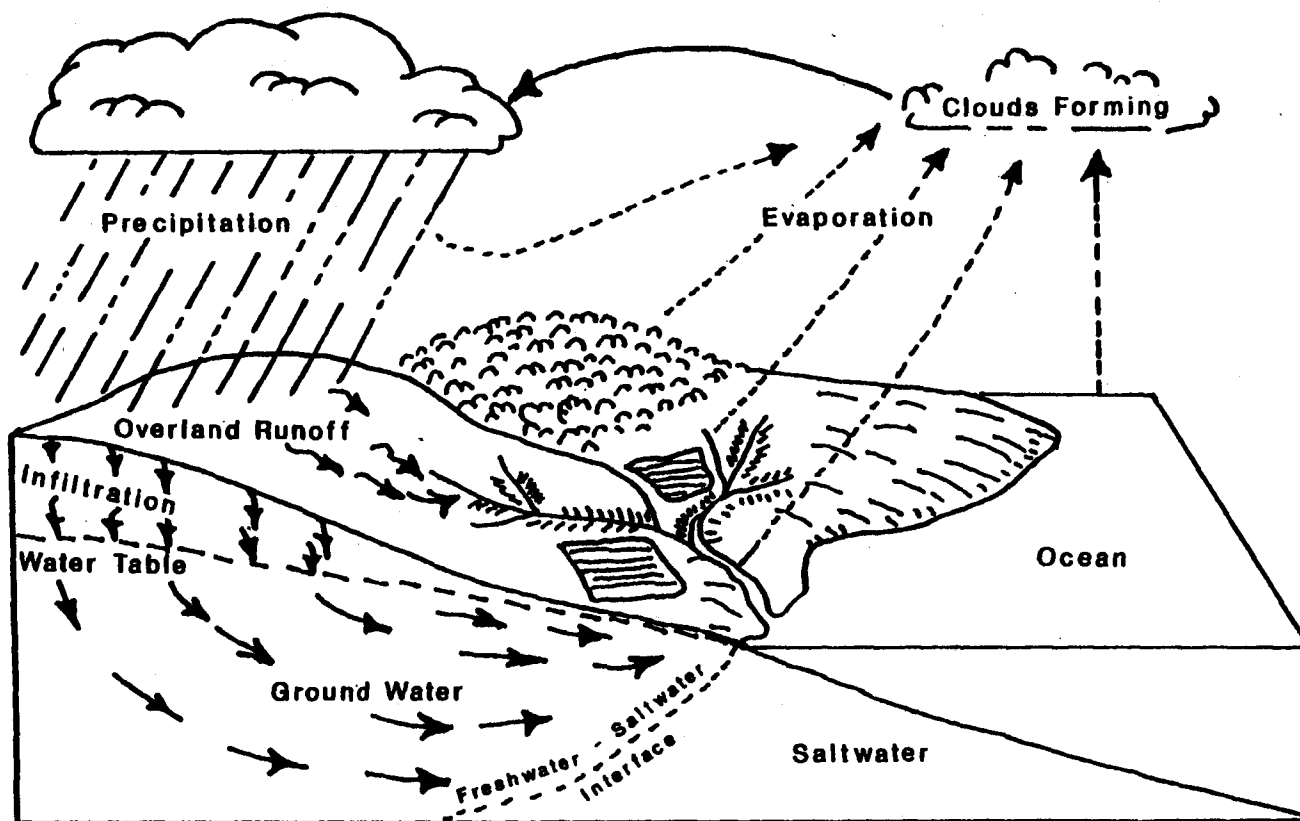
Figure 3. The Hydrologic Cycle (Heath, 1982).
