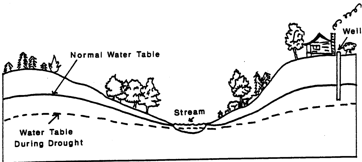
Figure 8. Hypothetical Sketch of the Seasonal Shape of the Water Table. The shape of the water table generally follows surface topography. During dry periods the water table falls, reducing stream flow and drying up some wells (modified after Tarbuck and Lutgens, 1984).
