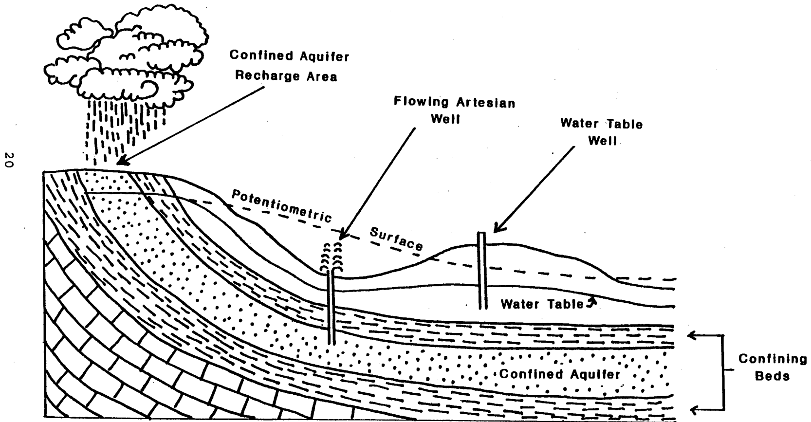
Figure 9. Geologic Section showing Confined and Unconfined Aquifers (modified after Tarbuck and Lutgens, 1984). See text for explanation.
