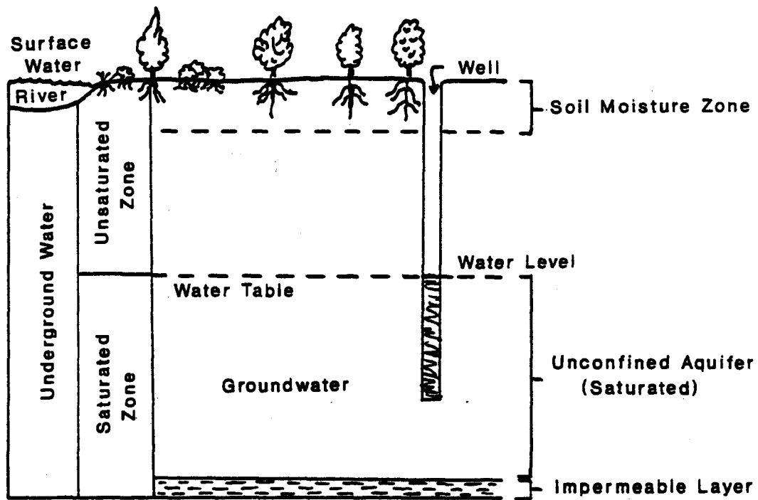
Figure 7. Vertical Distribution of Underground Water in a Typical Unconfined Aquifer (modified after Heath, 1982).
