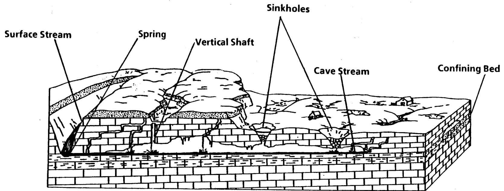
Figure 10. Block Diagram showing Surface and Subsurface Karst Features (modified after Currens and McGrain, 1979).
