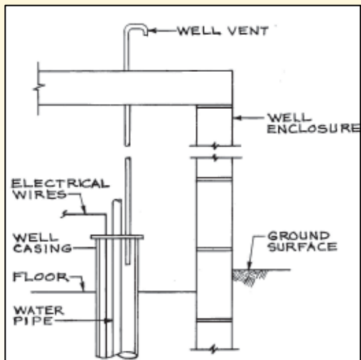
Figure 4. Recommended venting procedures for wells located in enclosed structures.
