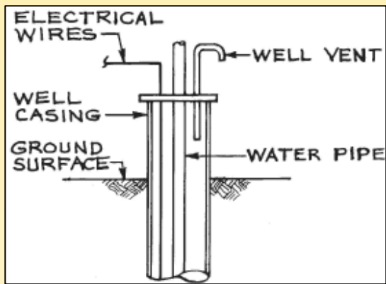
Figure 3. Recommended venting procedures for wells not enclosed in structures.
