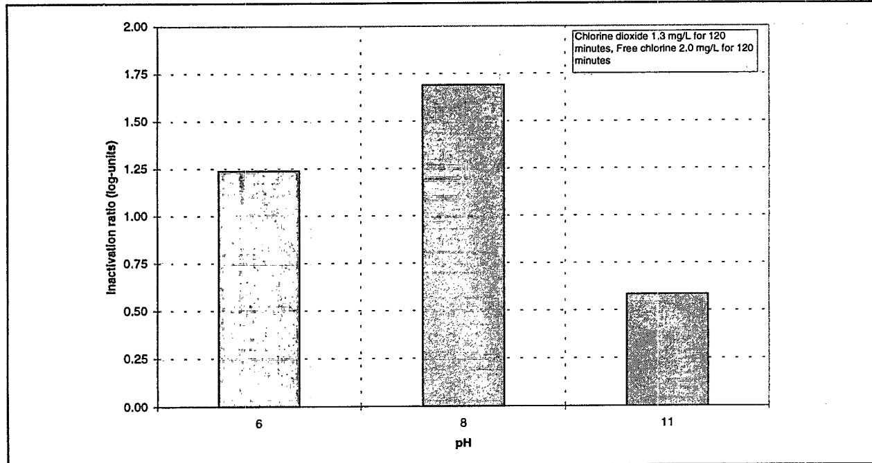
Figure 9-2. Inactivation of C. parvum Attributed to Synergistic Effects. Application of Chlorine Dioxide Followed by Free Chlorine
