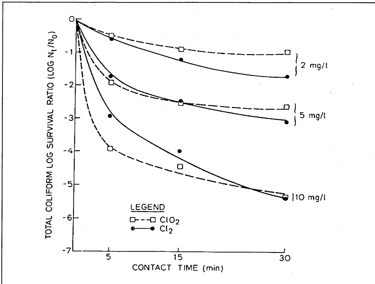
Figure 4-4. Comparison of Germicidal Efficiency of Chlorine Dioxide and Chlorine
