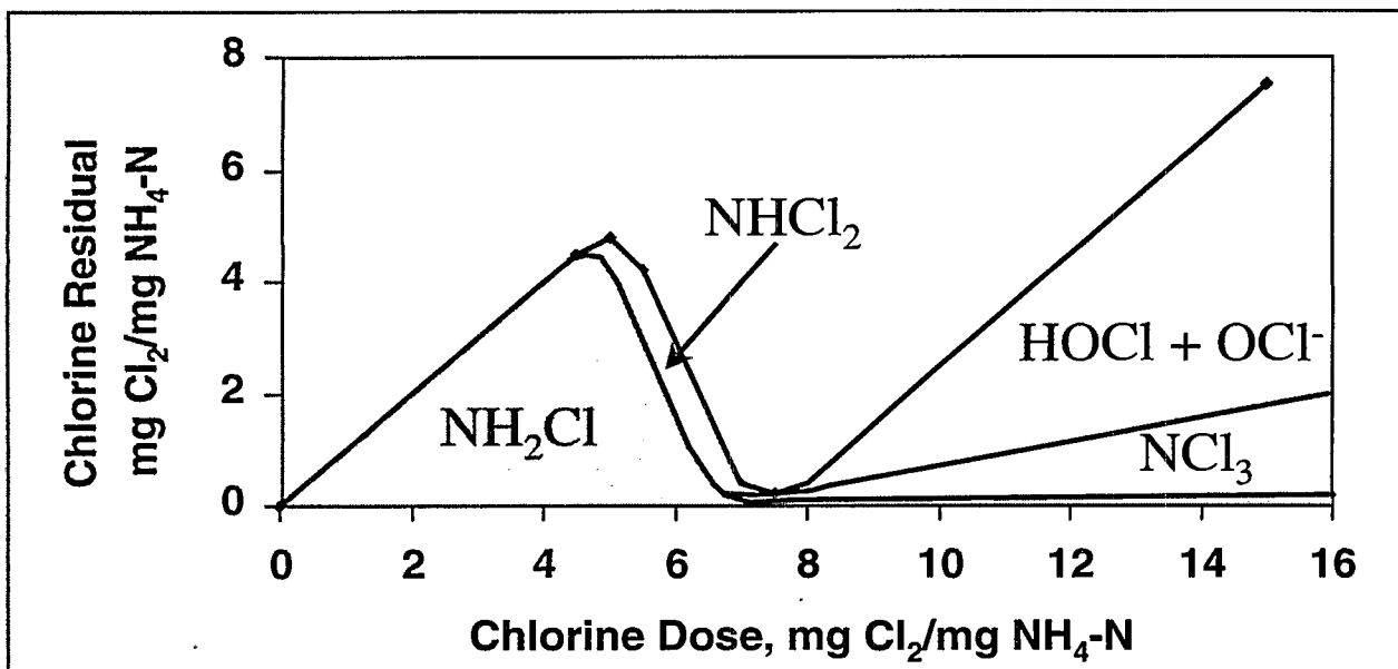
Figure 6-1. Theoretical Breakpoint Curve
