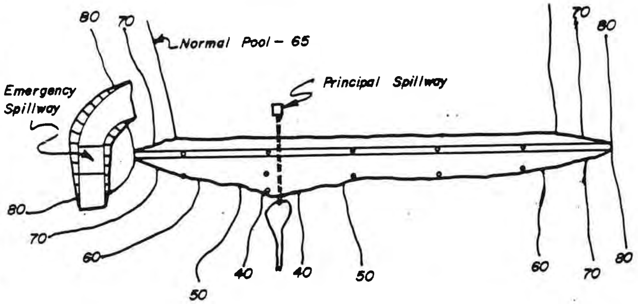
PLAN-BORING LAYOUT
