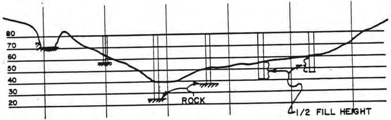
PROFILE THROUGH CREST BORINGS
