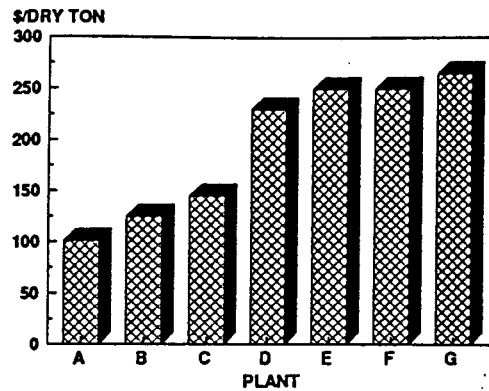
Figure 10. Comparison of costs for sludge processing using alkaline addition.
