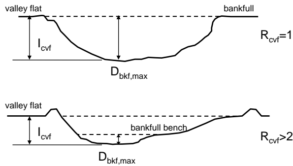
Figure 3.4 Relative incision.
