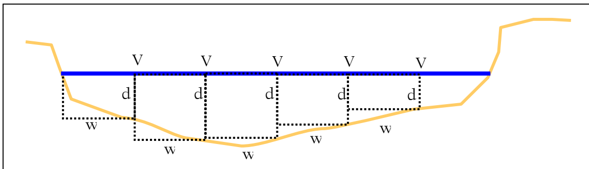
Stream cross-section showing intervals where water depth and velocity are measured. Flow will be calculated for each "box" (flow area for each box is d \times w ) and summed to obtain the flow for the entire stream.
