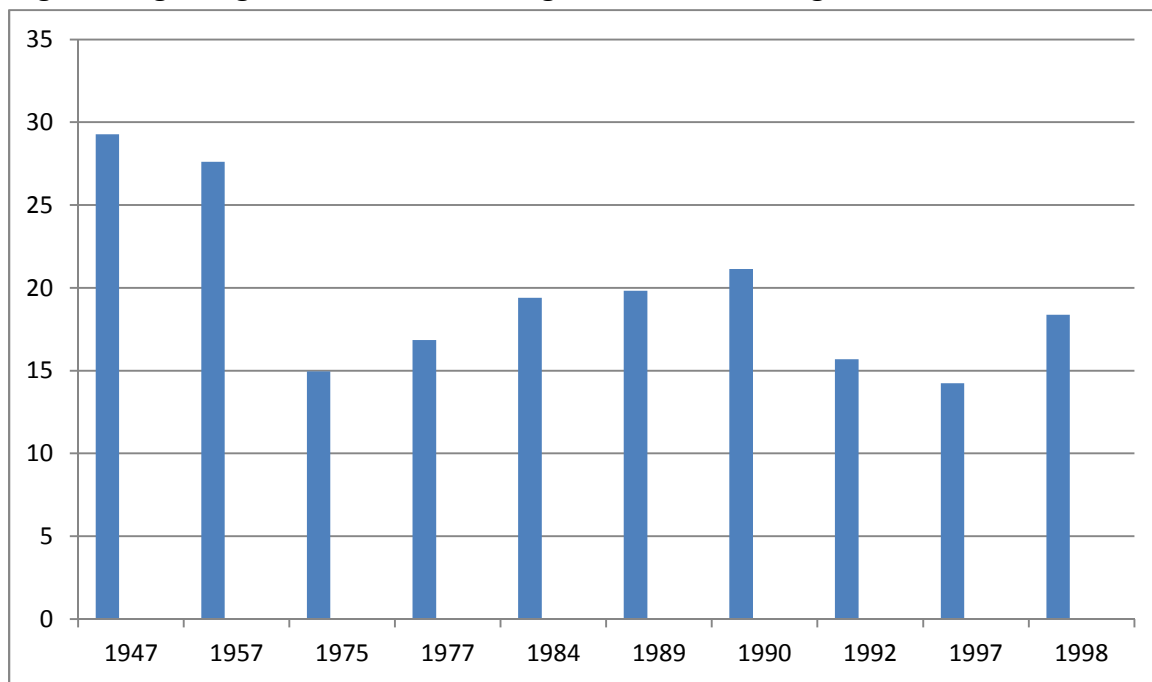
Highest Gage Heights in feet at USGS Gage 03281040 near Big Creek, KY, 1947-2000
