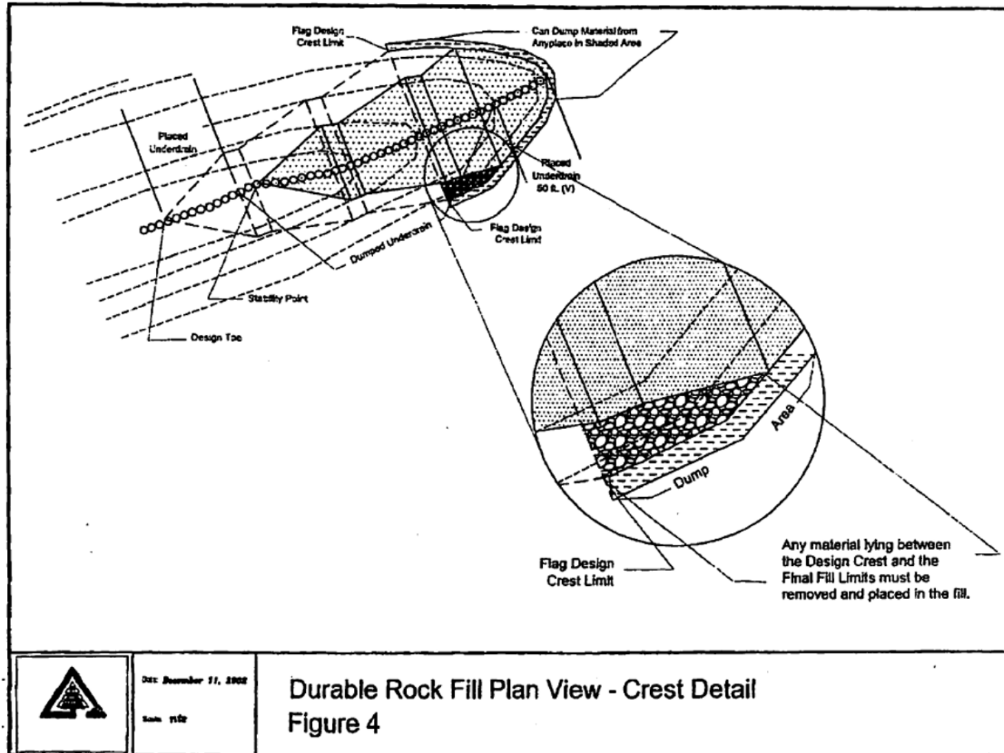
Drawing 4 – General Durable Rock Fill Plan View
