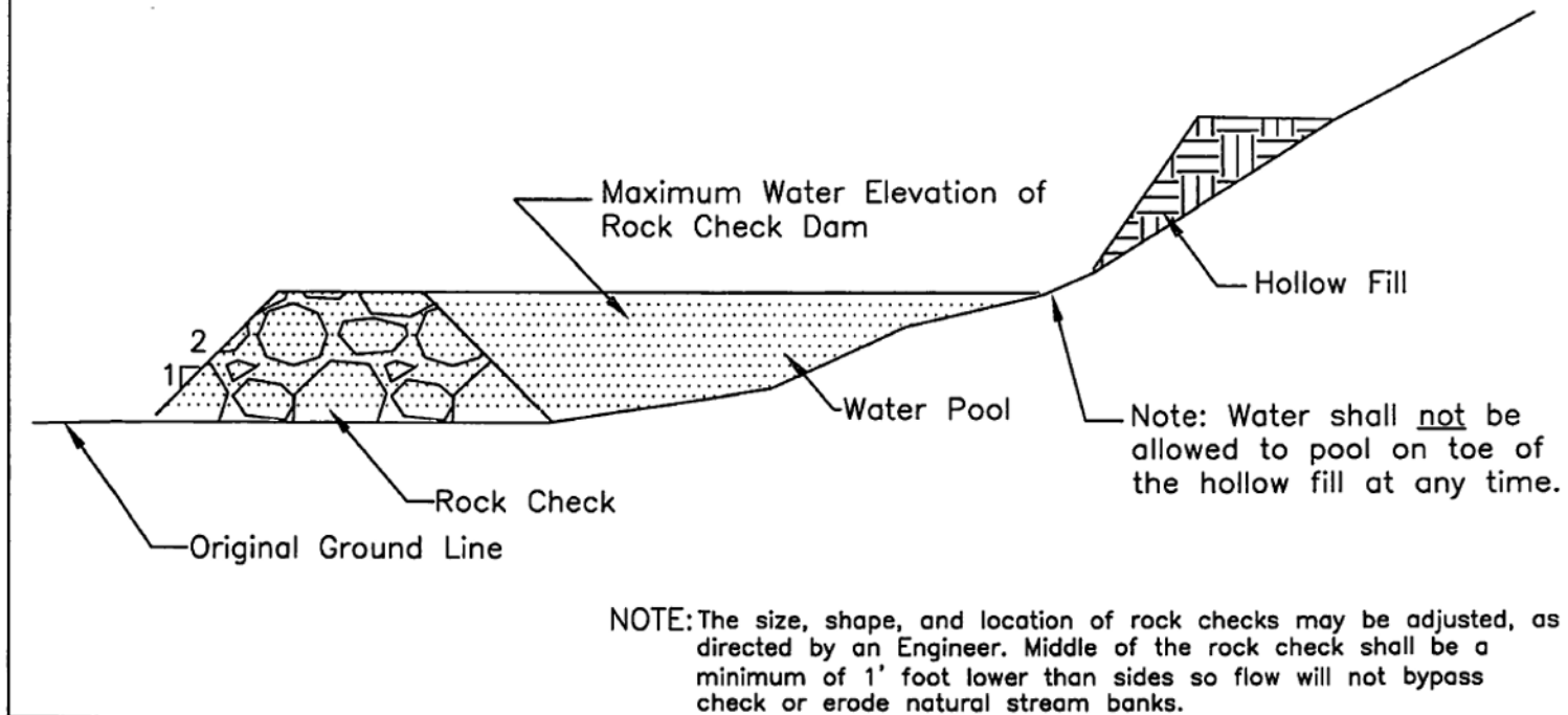
Drawing 5 – Rock Check Dam-Profile View
