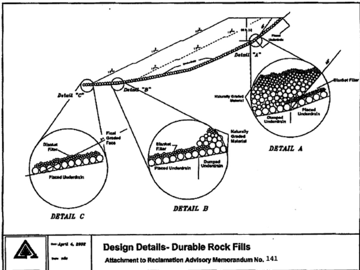
Drawing 3 – Design Details-Durable Rock Fills
