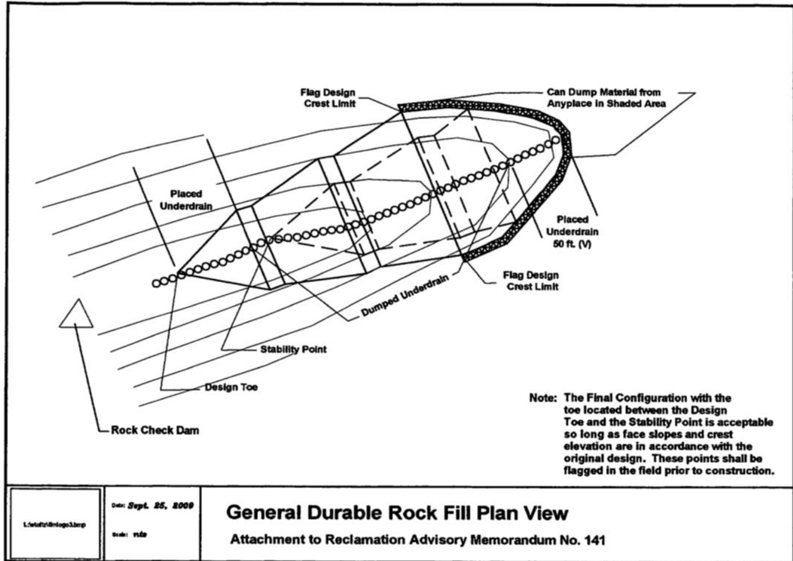
Drawing 1 – General Durable Rock Fill Plan View
