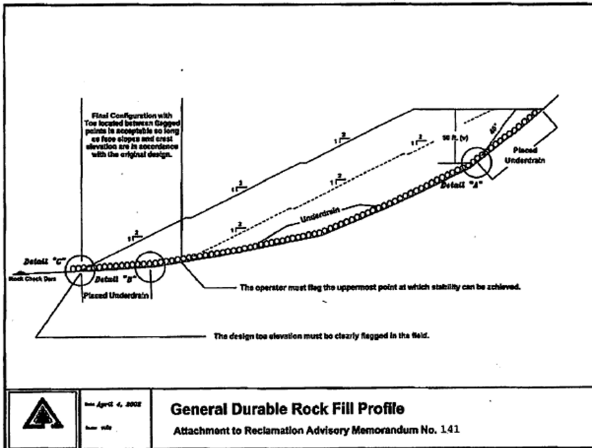
Drawing 2 – General Durable Rock Fill Profile
