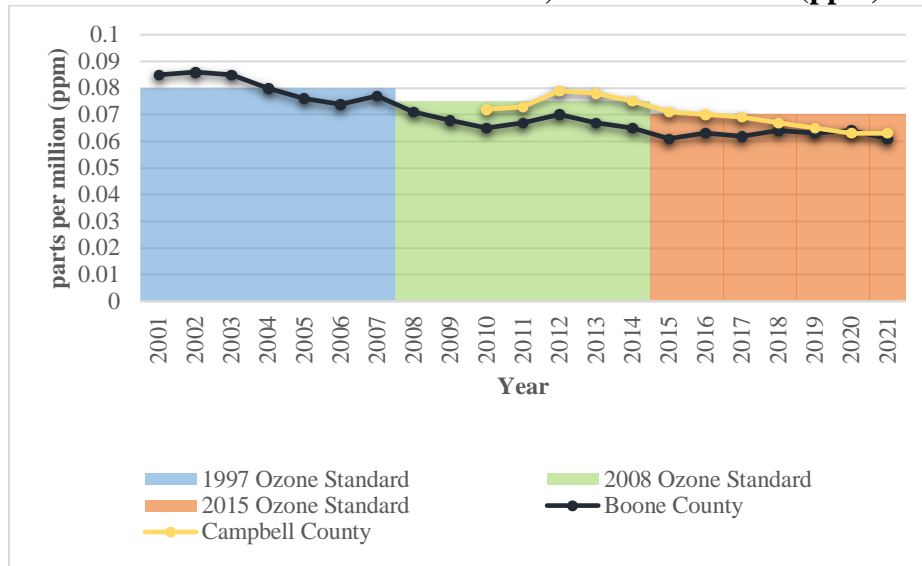
Figure 1 – 8-hour Ozone Design Values for the Kentucky Portion of the Cincinnati-Hamilton, OH-KY-IN Area (ppm)
