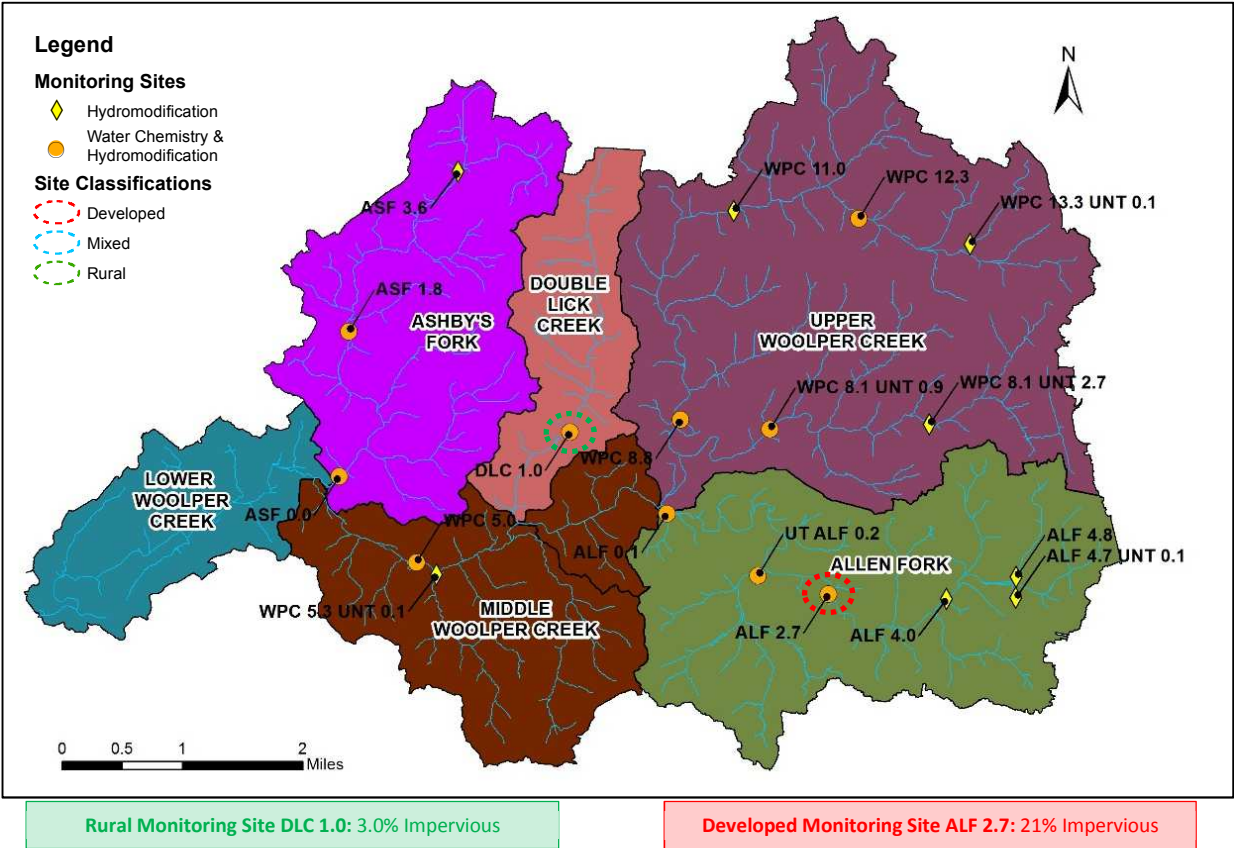
Figure 4-9: Level logger data locations for an undeveloped site (DLC 1.0) and a developed site (ALF 2.7).
