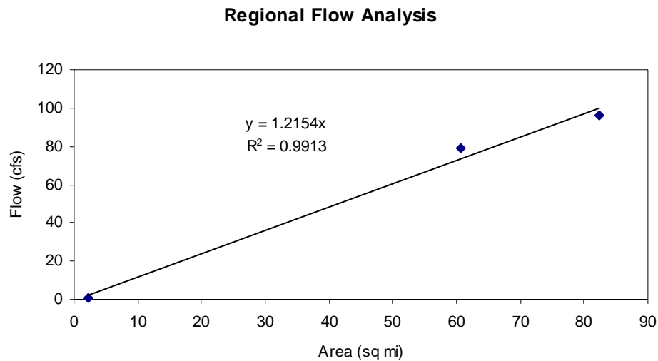
Figure 5. Relationship Between Basin Area and the Critical TMDL Flow
