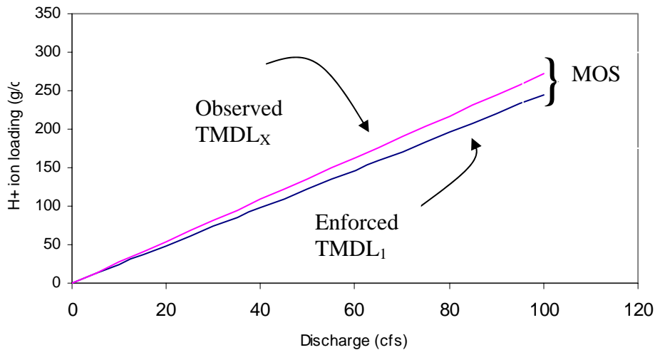
Figure 4. Relationship Between Discharge and Maximum Ion Load for a pH of 6.0
