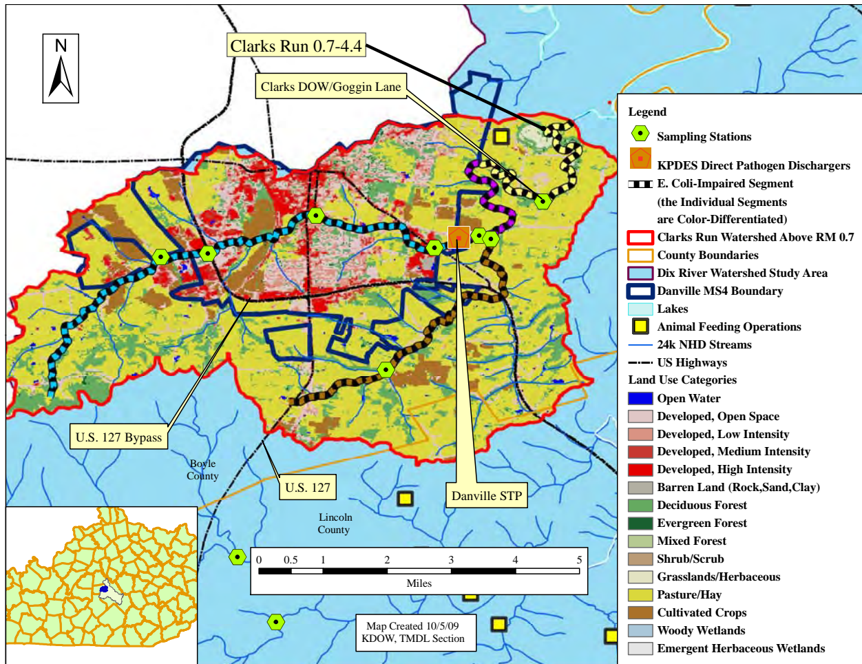
Figure 8.59 Clarks Run RM 0.7-4.4
