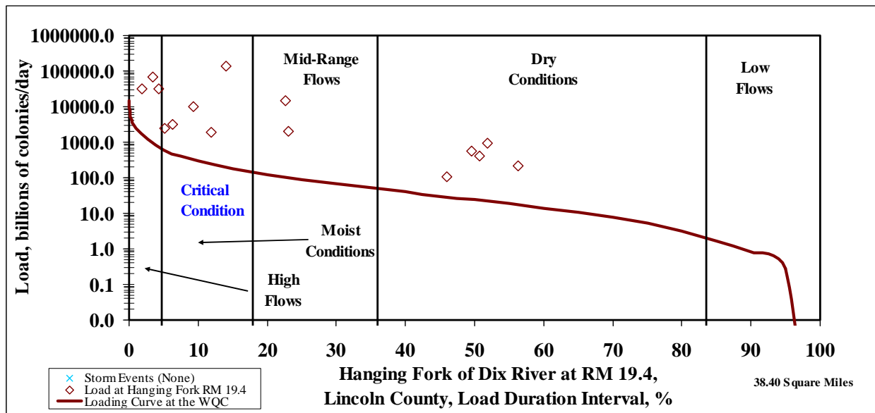
Figure 8.31 LDC for Hanging Fork RM 15.85-24.15
