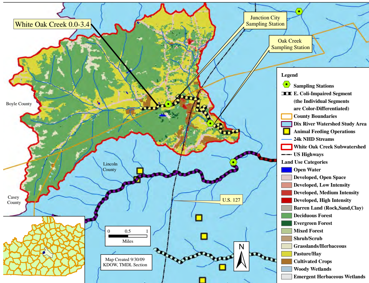
Figure 8.40 White Oak Creek RM 0.0-3.4
