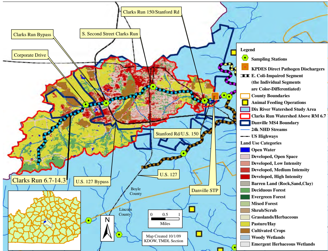
Figure 8.49 Clarks Run RM 6.7-14.3
