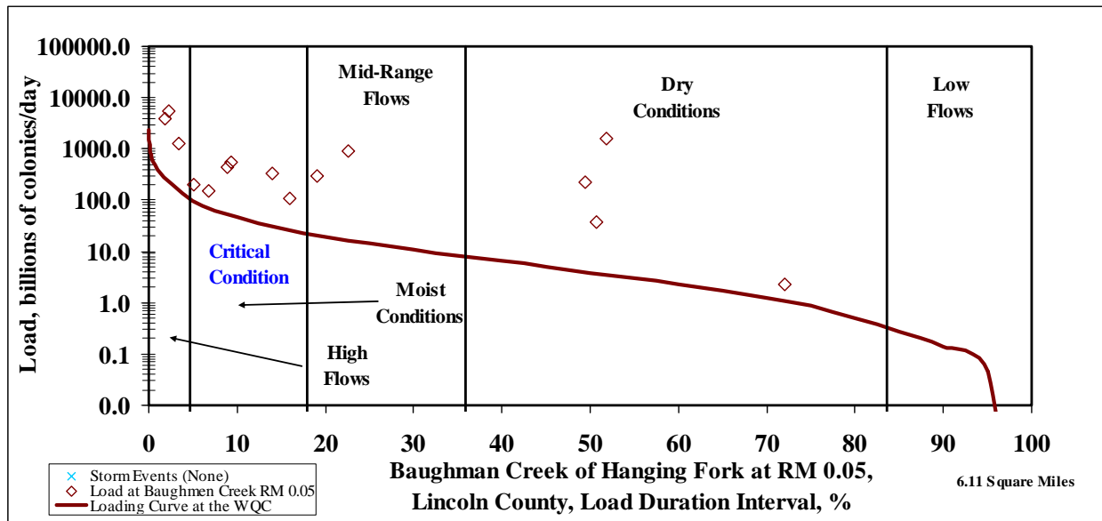
Figure 8.25 LDC for Baughman Creek RM 0.0-4.6
