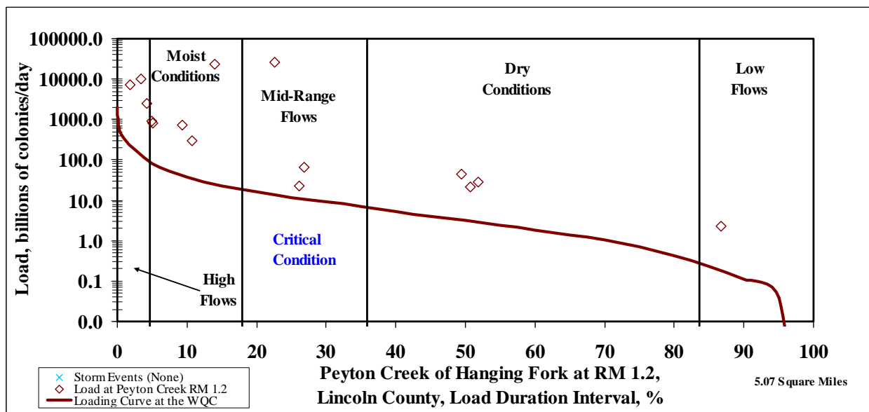
Figure 8.35 LDC for Peyton Creek RM 0.0-4.1
