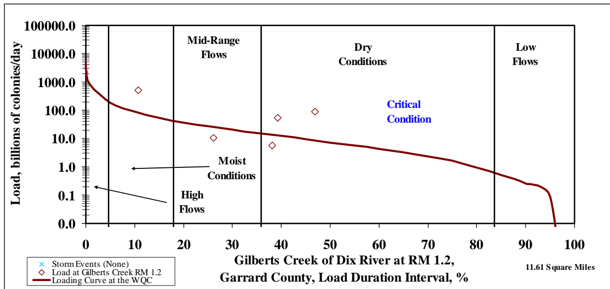
Figure 8.11 LDC for Gilberts Creek 0.0-1.25
