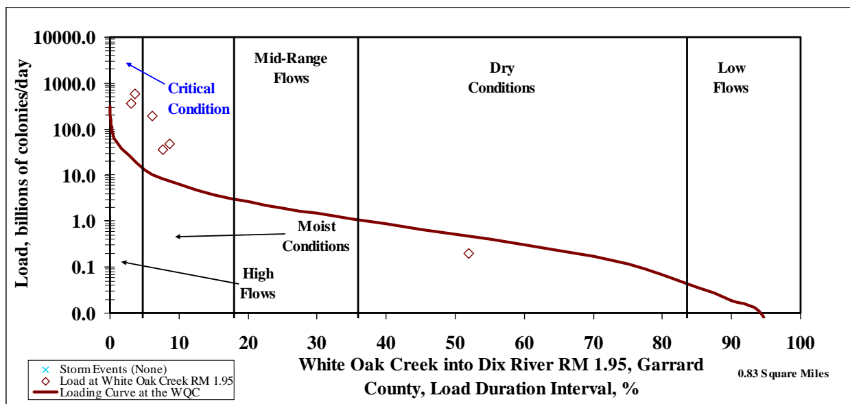
Figure 8.16 LDC for White Oak Creek 0.0-2.8
