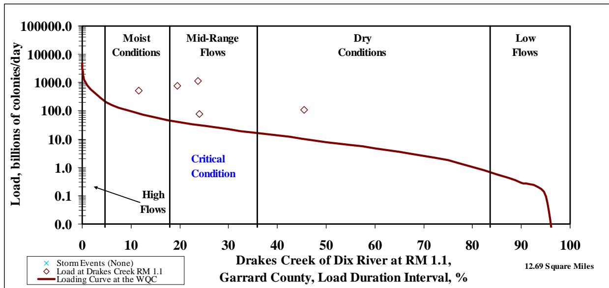
Figure 8.9 LDC for Drakes Creek 1.15-7.6
