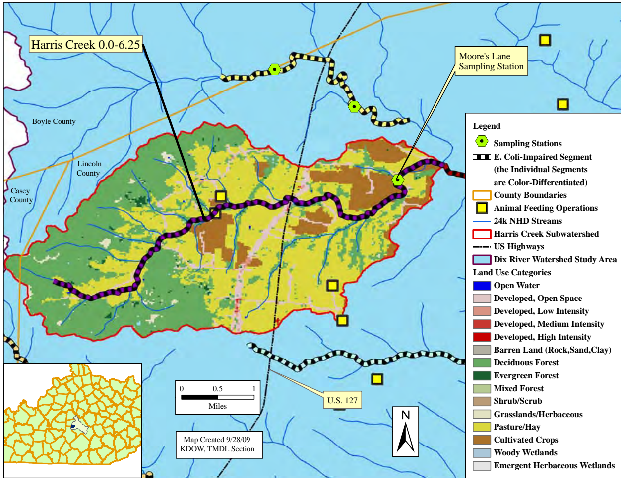
Figure 8.38 Harris Creek RM 0.0-6.25
