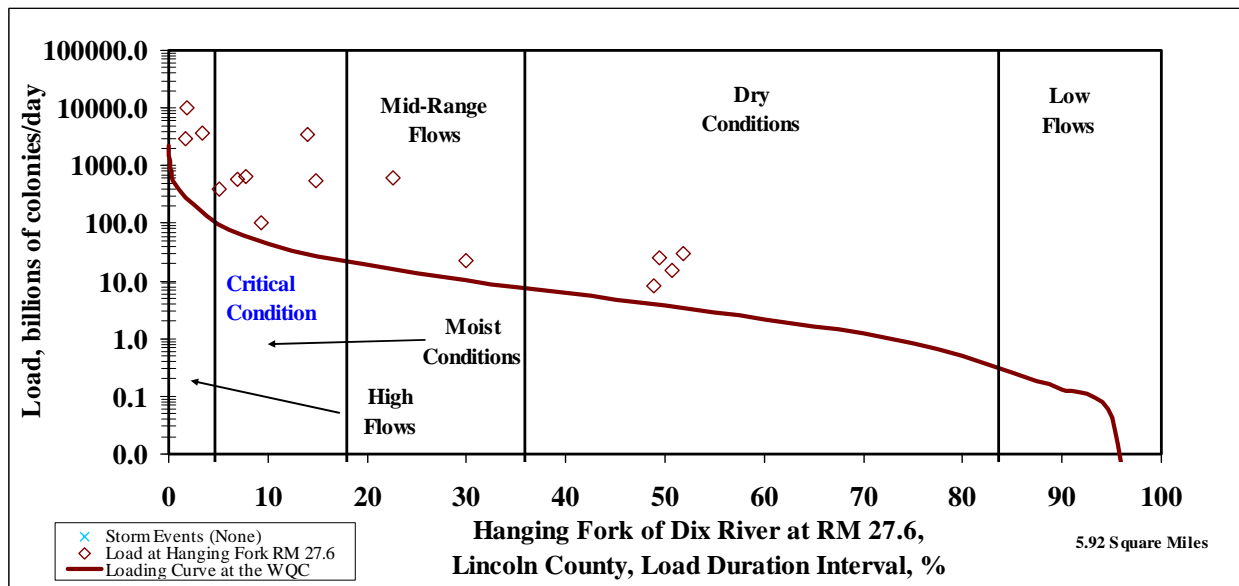
Figure 8.23 LDC for Hanging Fork RM 27.6-32.2
