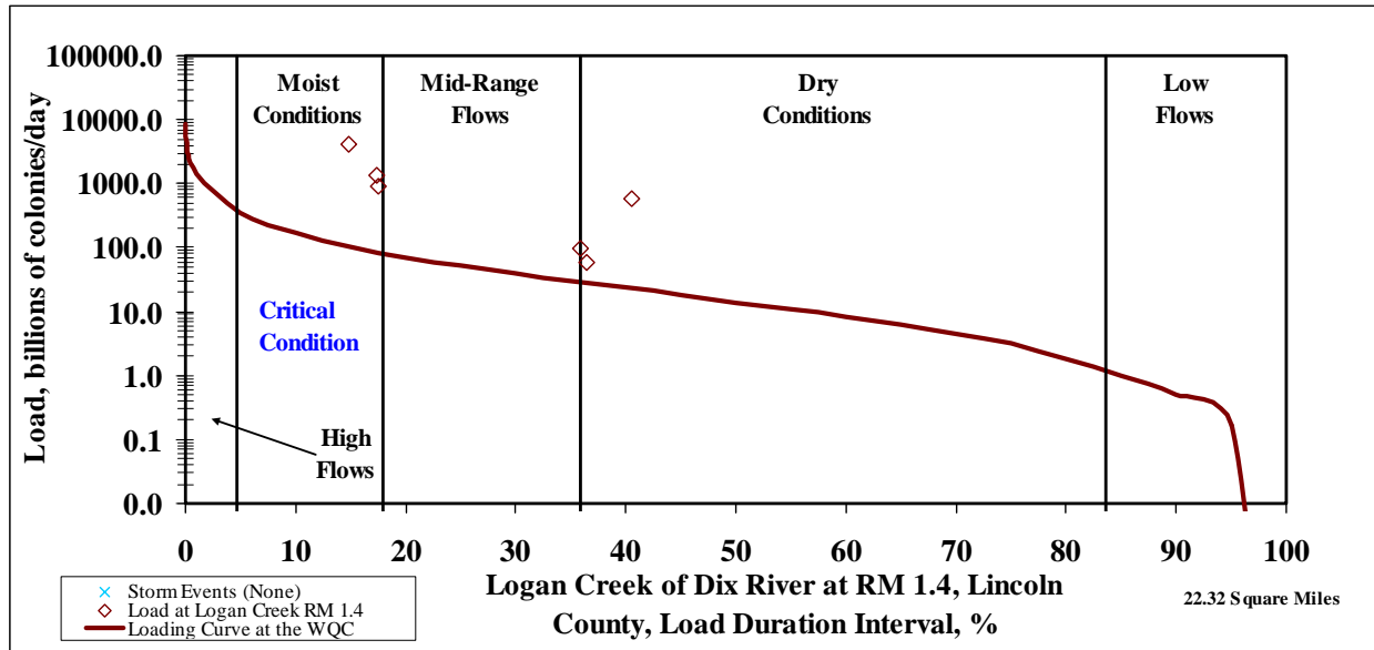
Figure 8.13 LDC for Logan Creek RM 0.0-3.15
