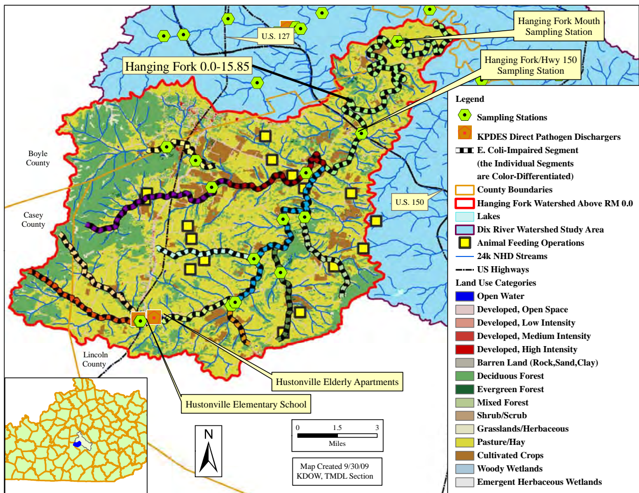
Figure 8.45 Hanging Fork RM 0.0-15.85
