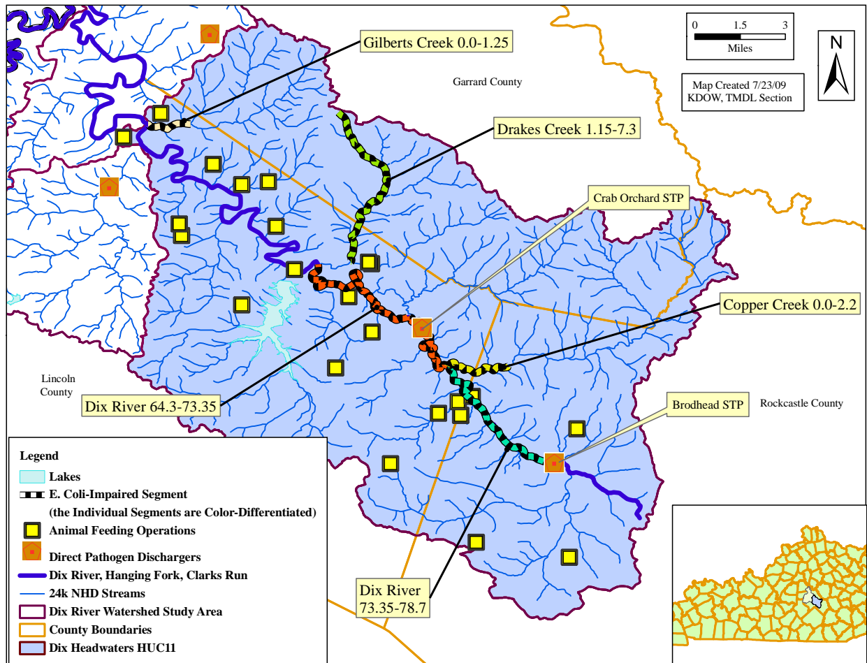
Figure 8.1 Dix Headwaters HUC11
