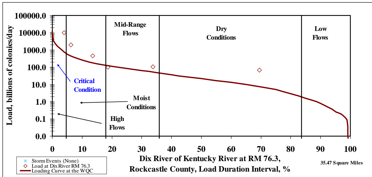
Figure 8.5 LDC for Dix River RM 73.35-78.7
