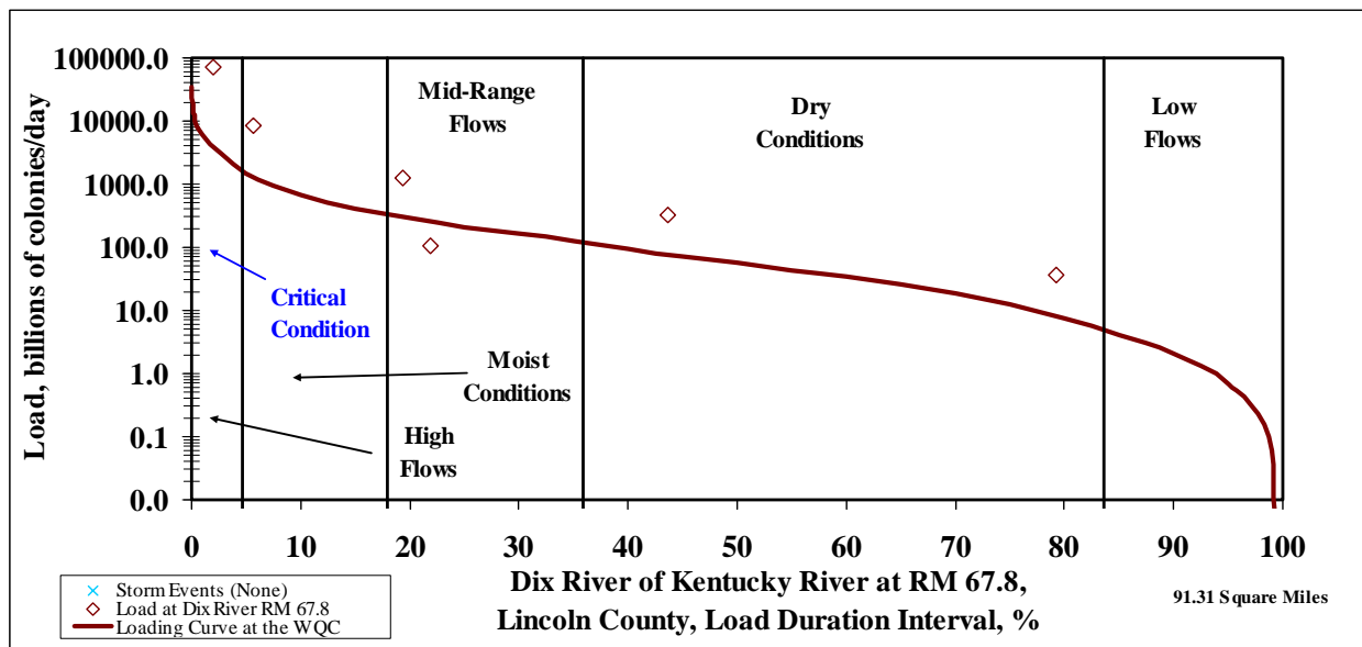
Figure 8.7 LDC for Dix River 64.3-73.35
