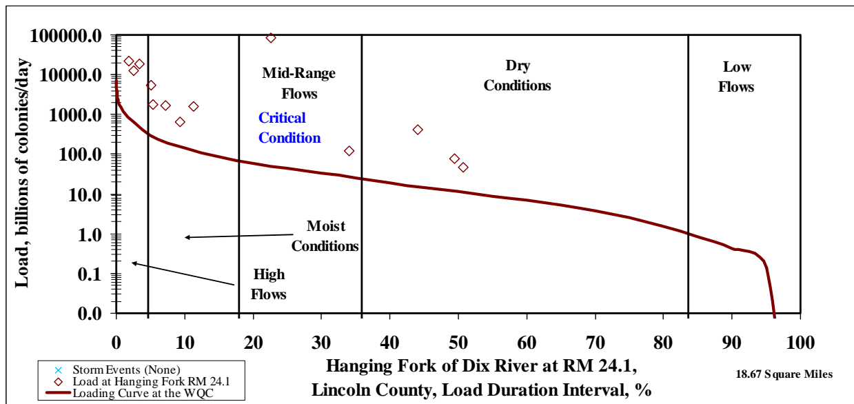
Figure 8.27 LDC for Hanging Fork RM 24.15-27.6
