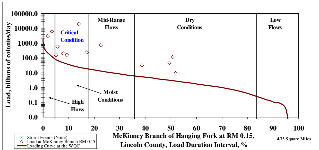
Figure 8.29 LDC for McKinney Branch RM 0.0-1.9
