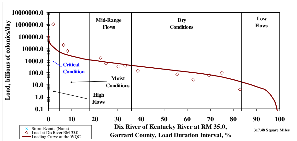
Figure 8.20 LDC for Dix River RM 33.3-36.1
