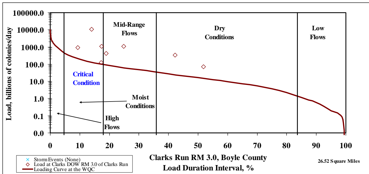
Figure 8.60 LDC for Clarks Run RM 0.7-4.4
