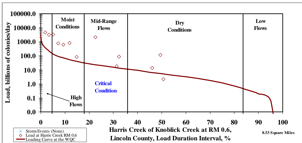
Figure 8.39 LDC for Harris Creek RM 0.0-6.25
