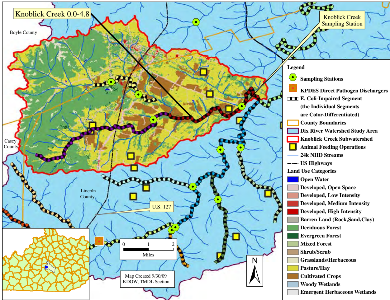
Figure 8.43 Knoblick Creek RM 0.0-4.8
