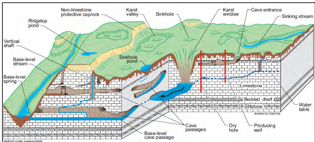
Figure 3. Karst Aquifer Block Diagram (Currens, 2001)
