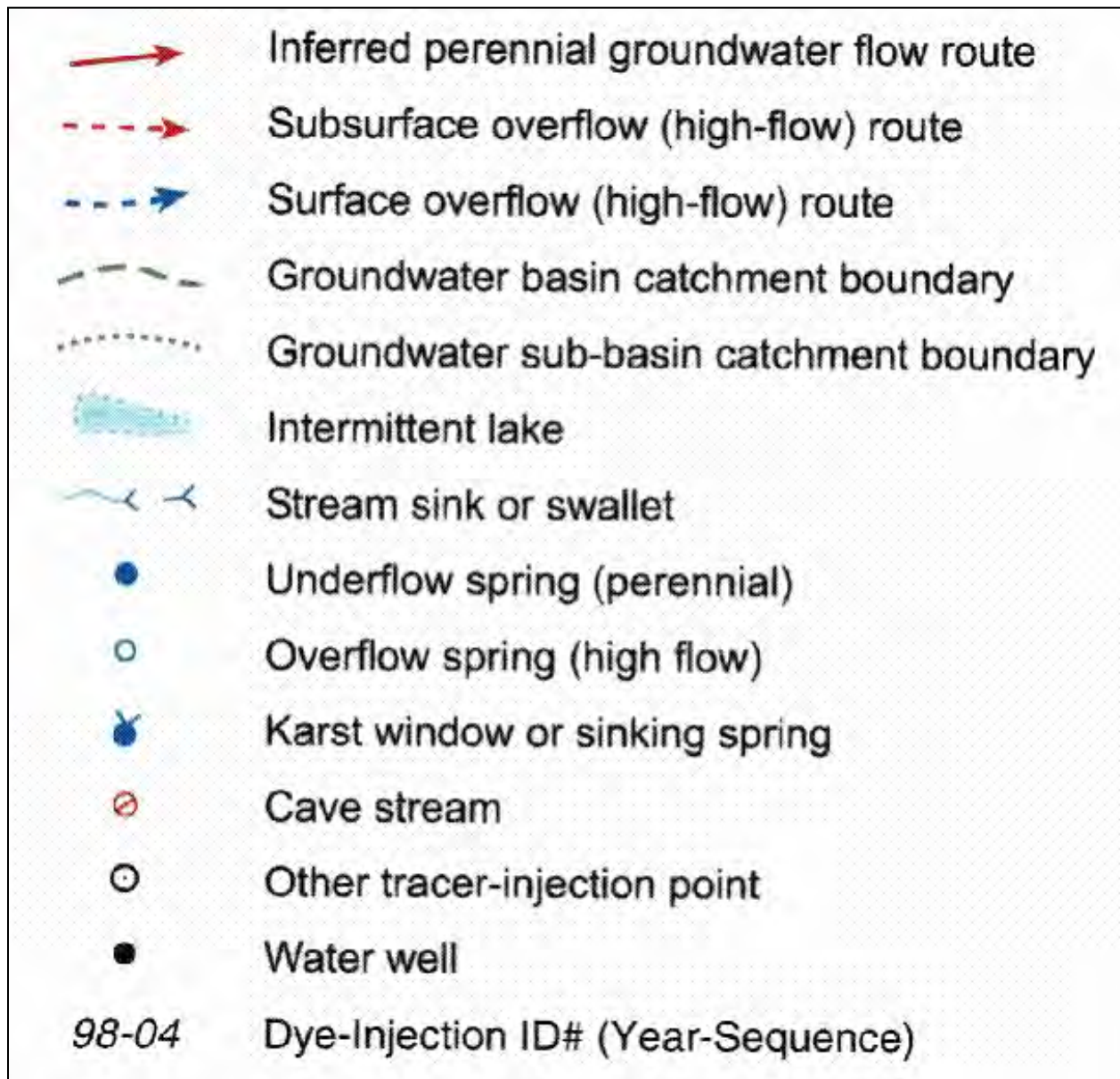
Figure 5. Karst Atlas Map Legend
