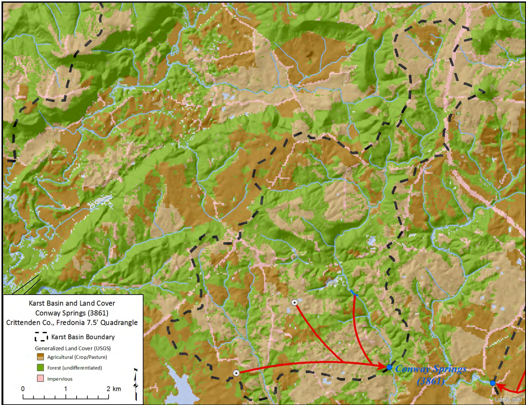
Figure 30. Conway Springs Karst Basin and Land Cover Map (WAH-Full Support, PCR-Full Support)
