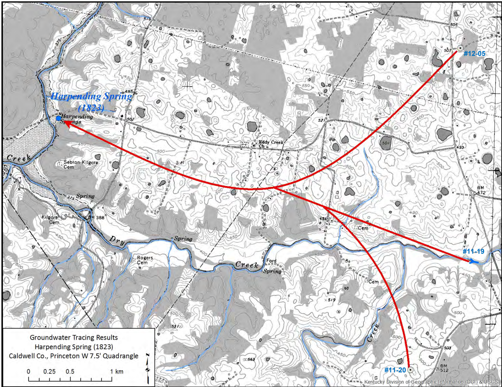
Figure 10. Harpending Spring Tracer Map
