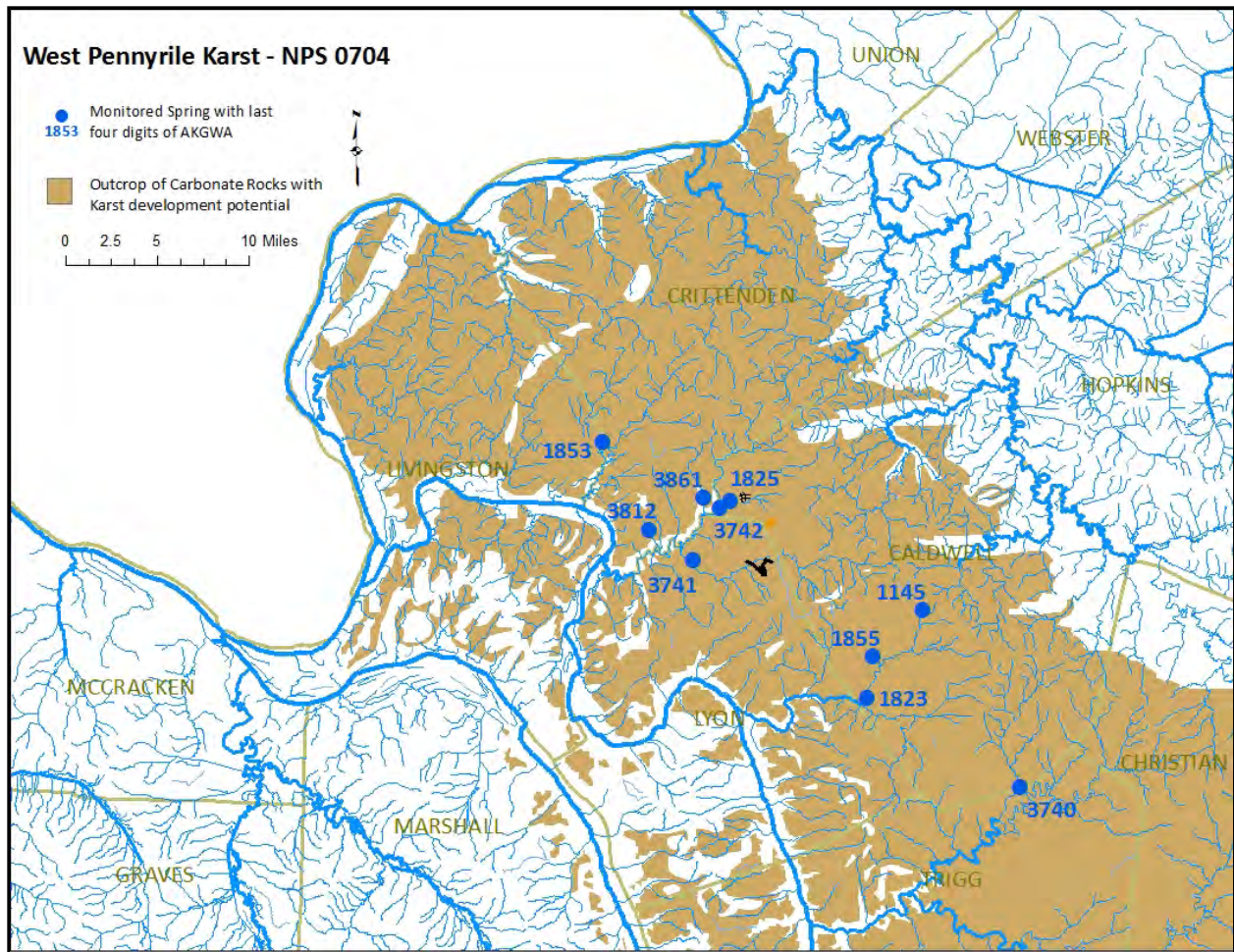
Figure 2. Map showing Springs to be monitored.
