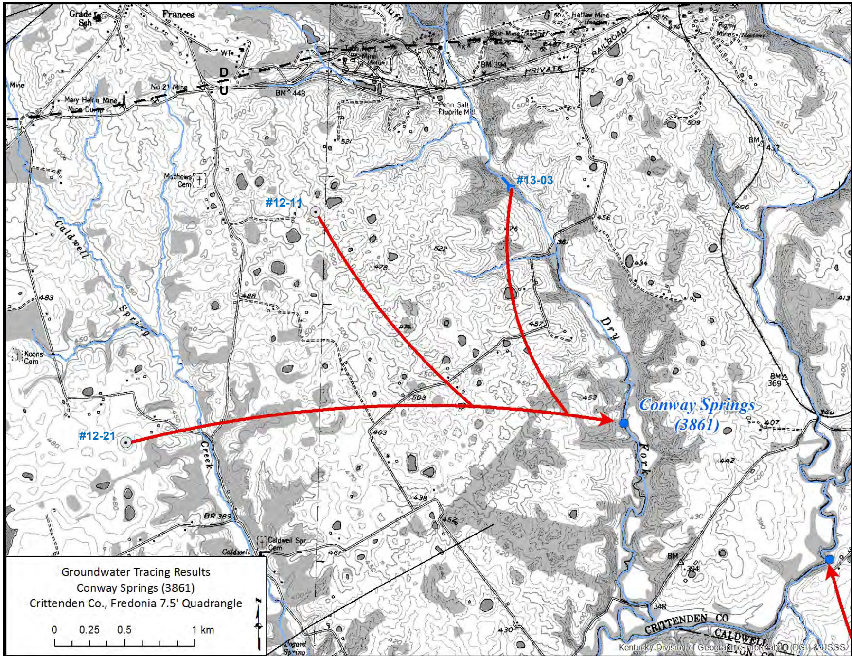
Figure 17. Conway Springs Tracer Map
