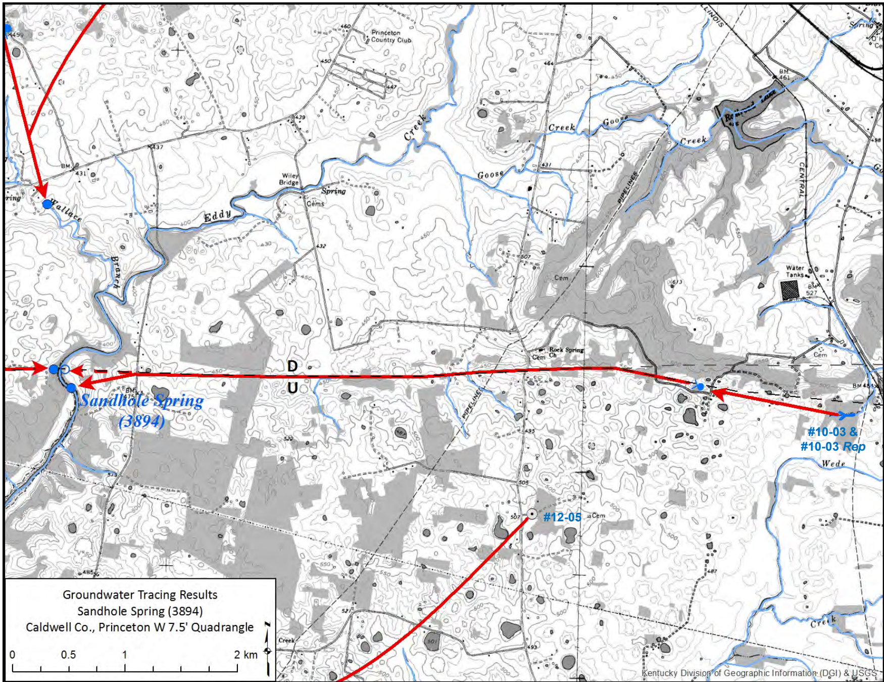
Figure 11. Sandhole Spring Tracer Map
