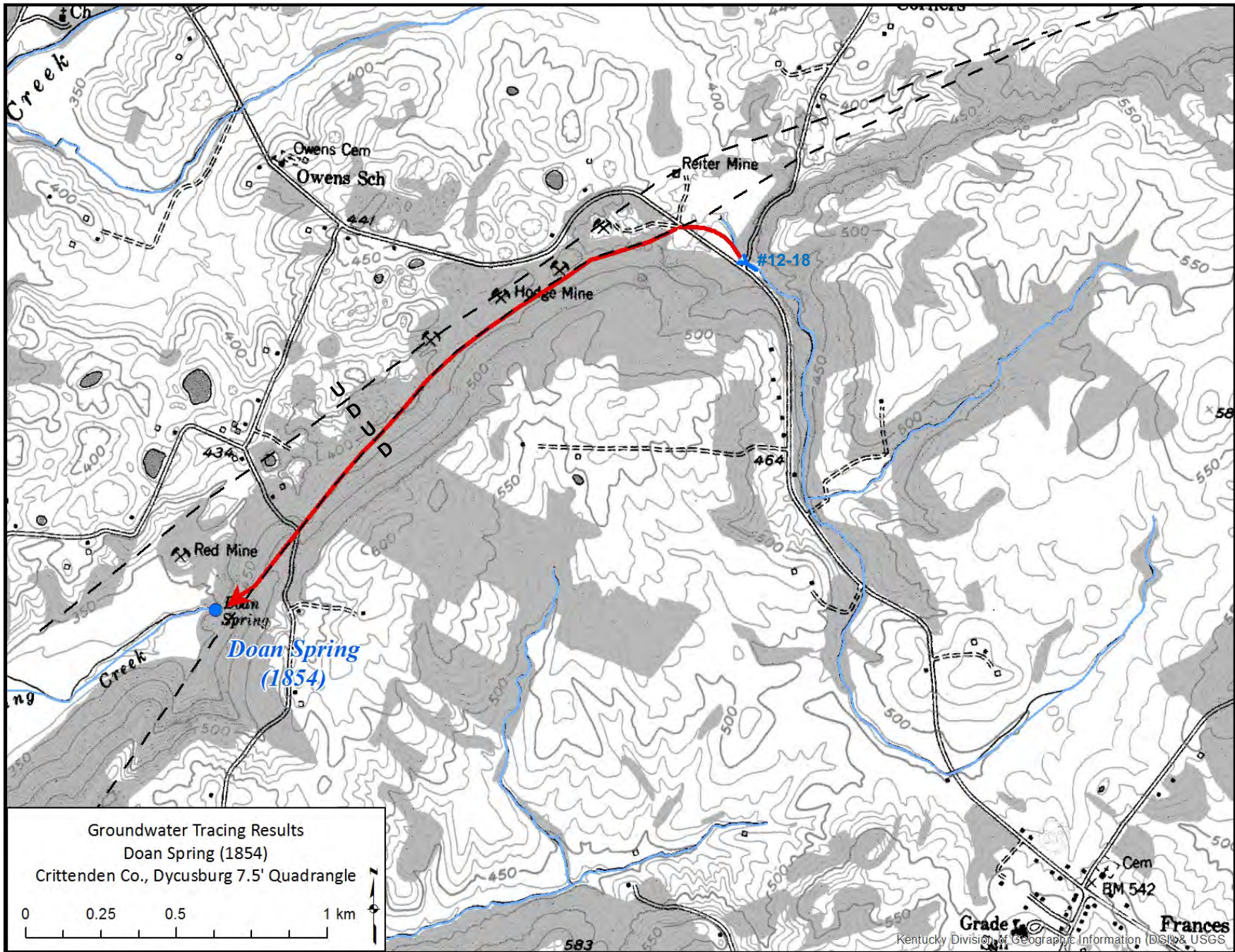
Figure 18. Doan Spring Tracer Map
