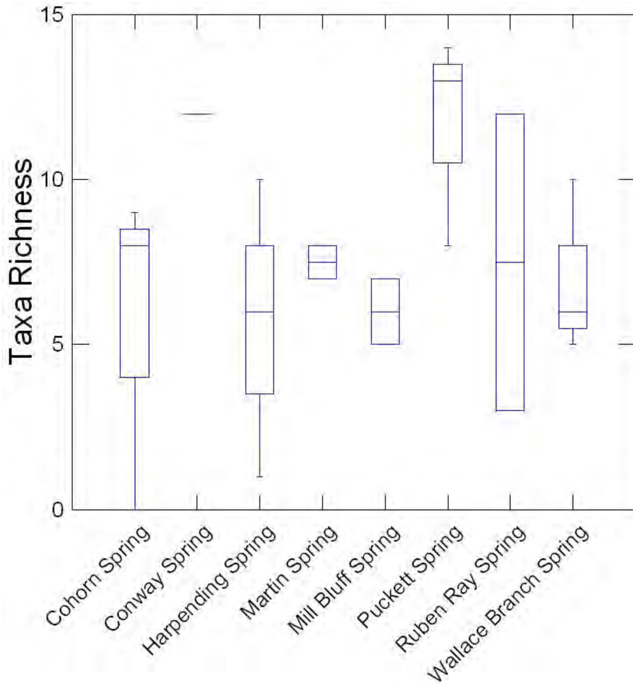
Figure 33. Mean Taxa Richness per Spring
