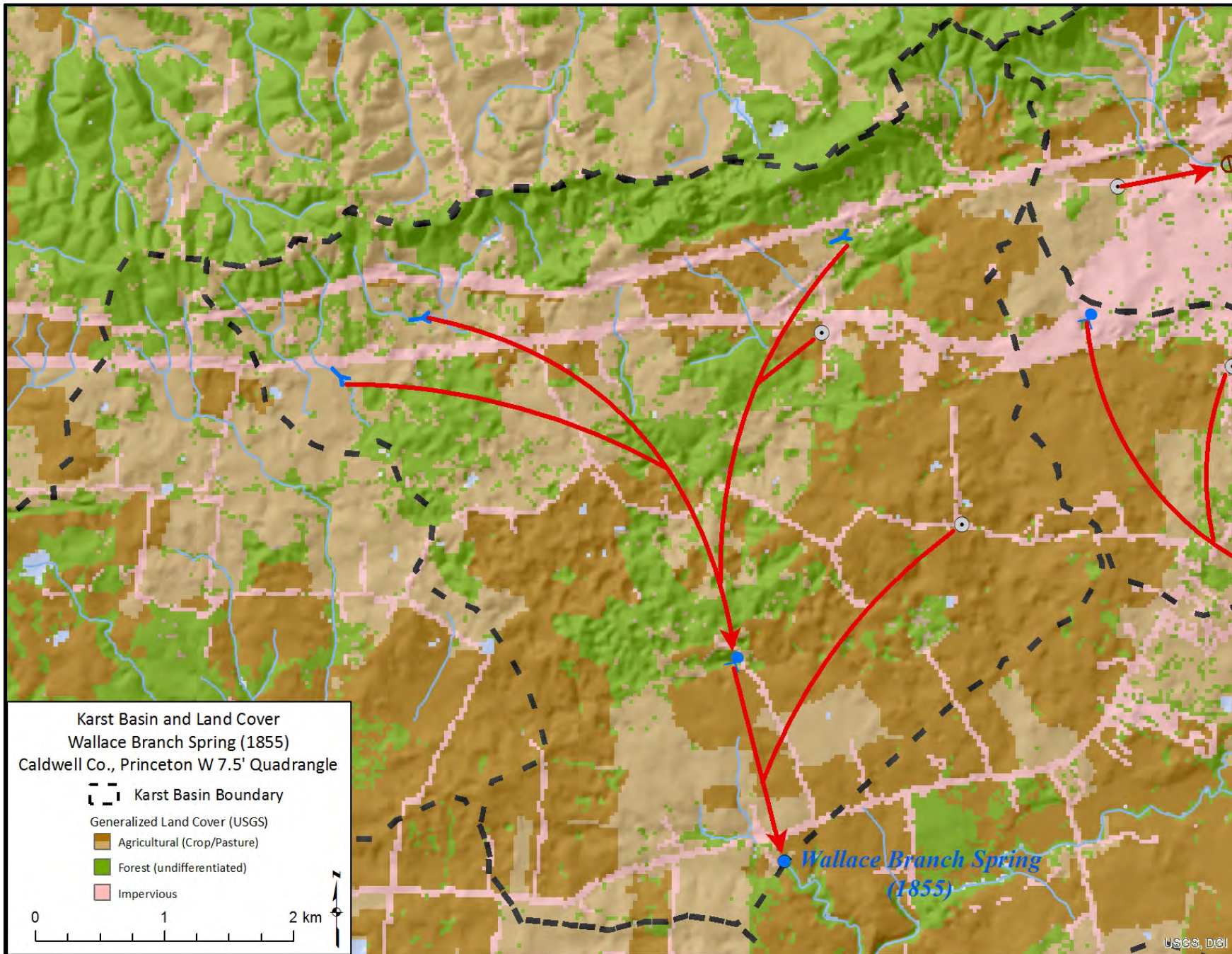
Figure 25. Wallace Branch Spring Karst Basin and Land Cover Map (WAH-Full Support, PCR-Partial Support)
