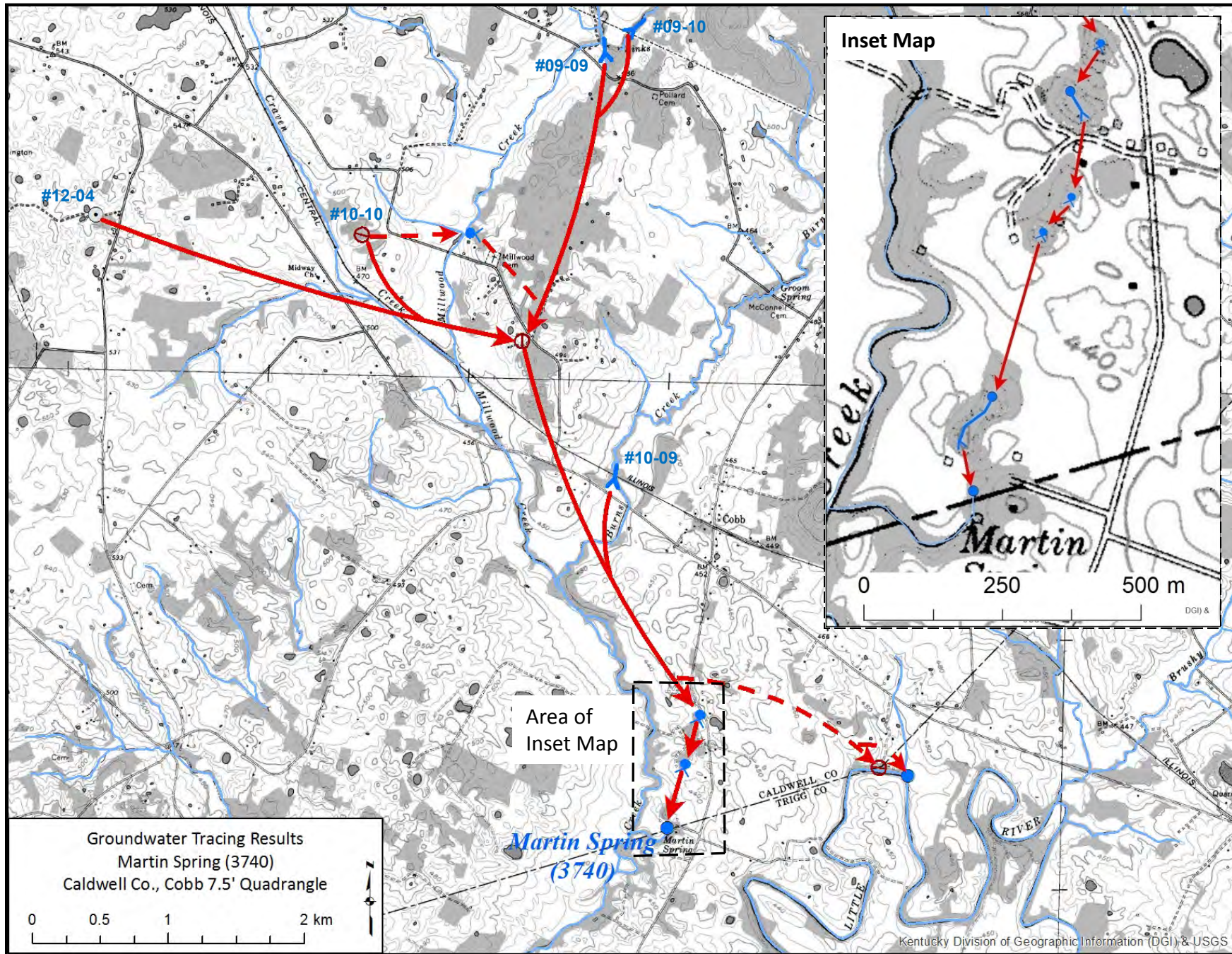
Figure 9. Martin Spring Tracer Map
