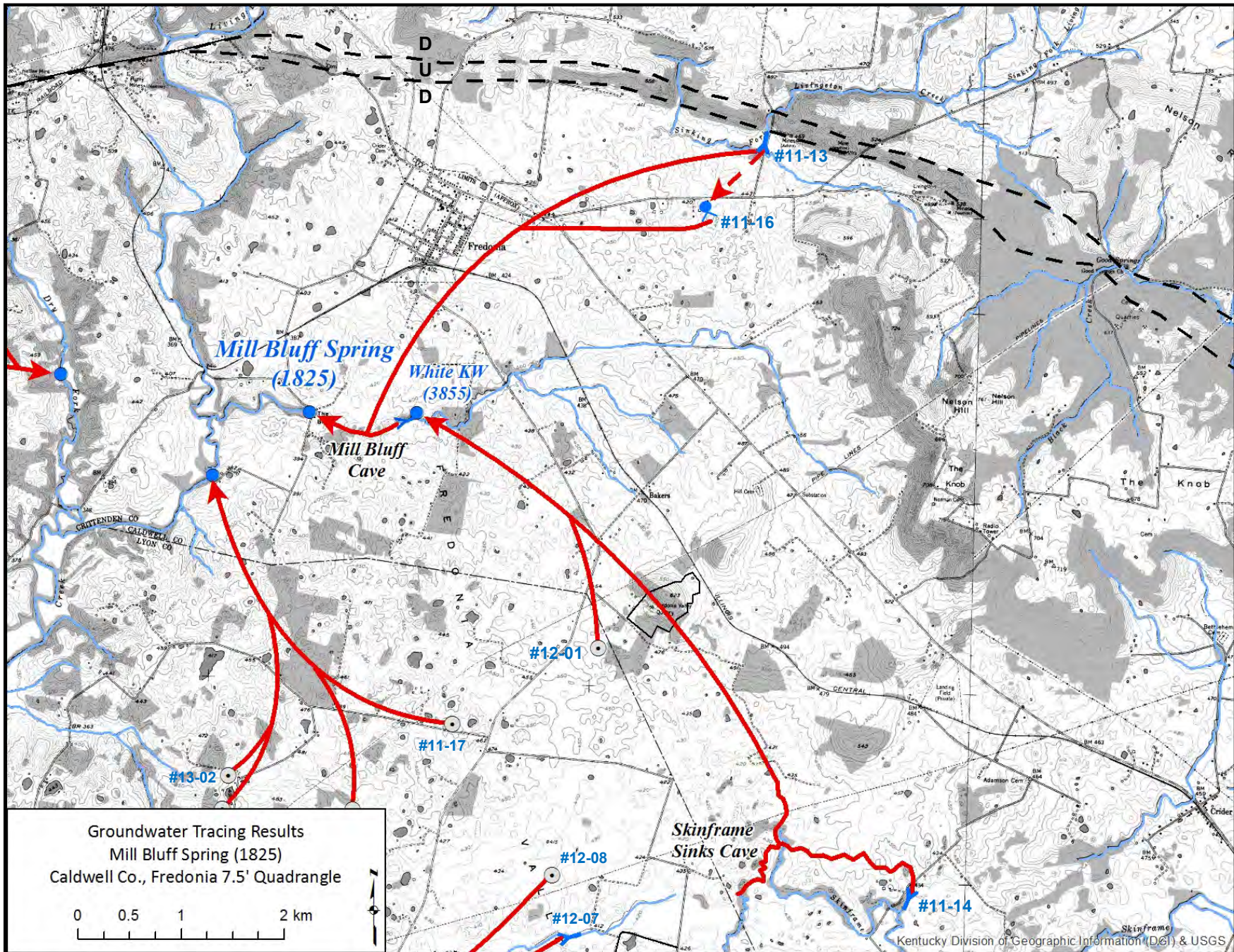
Figure 16. Mill Bluff Spring Tracer Map
