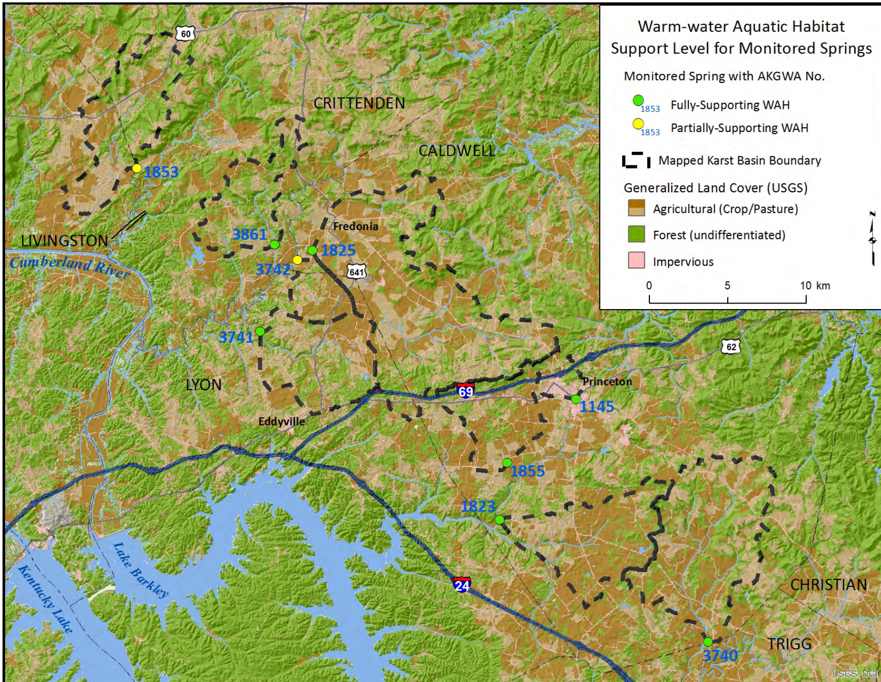
Figure 22. Monitored Springs WAH Support Level
