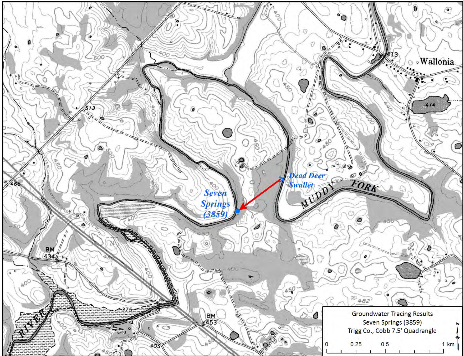
Figure 8. Seven Springs Tracer Map
