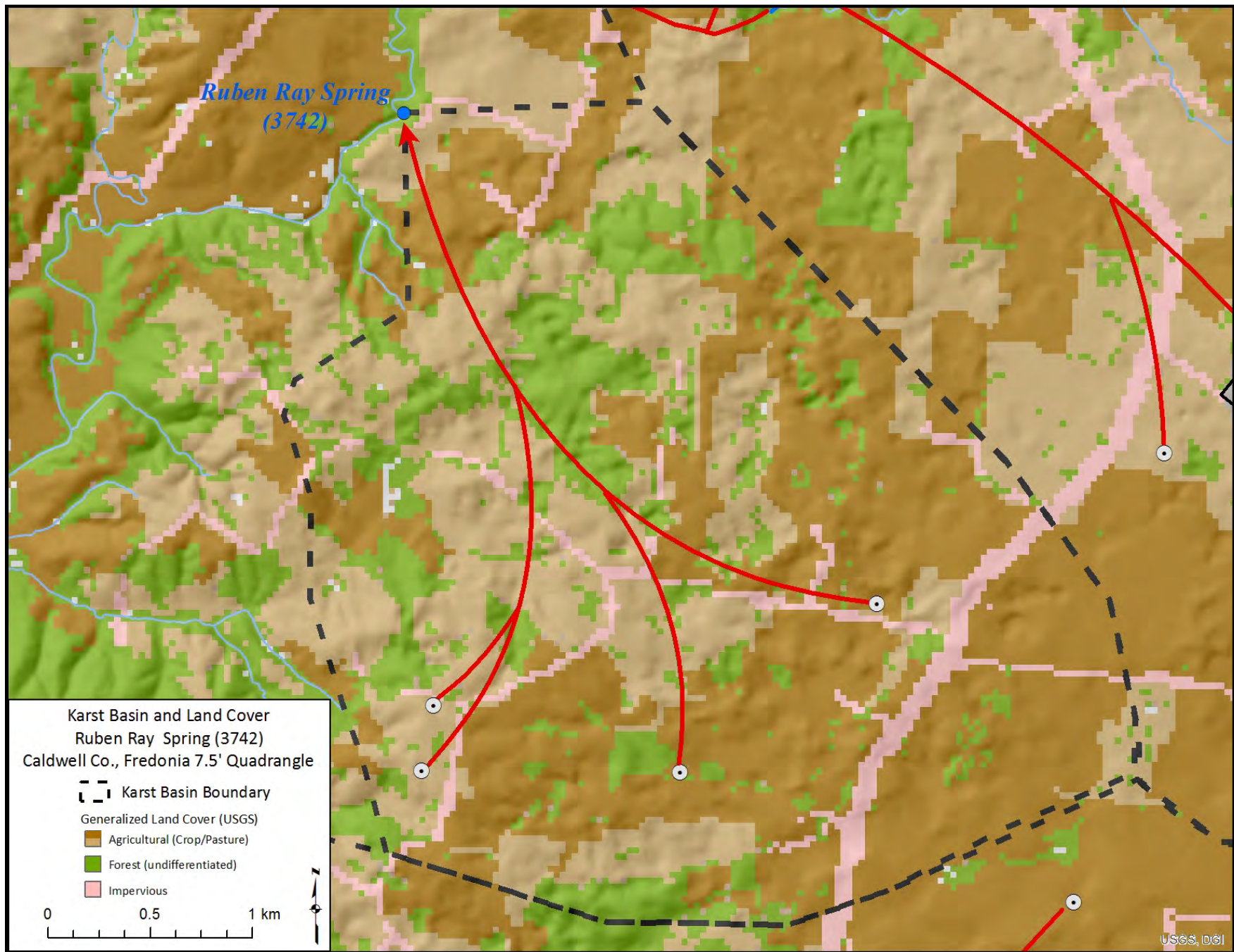
Figure 31. Ruben Ray Spring Karst Basin and Land Cover Map (WAH-Partial Support, PCR-Full Support)
