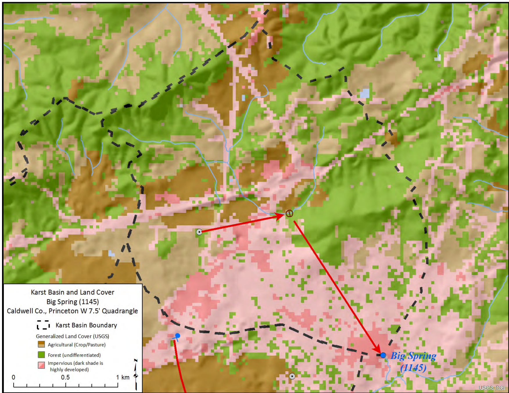
Figure 32. Big Spring Karst Basin and Land Cover Map (WAH-Full Support, PCR-Partial Support)
