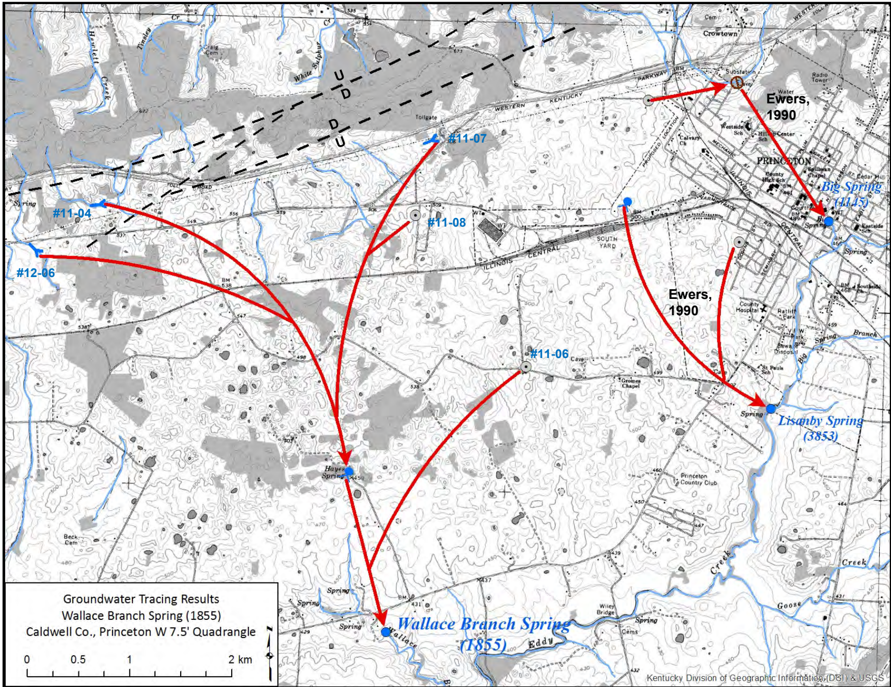
Figure 13. Wallace Branch Spring Tracer Map
