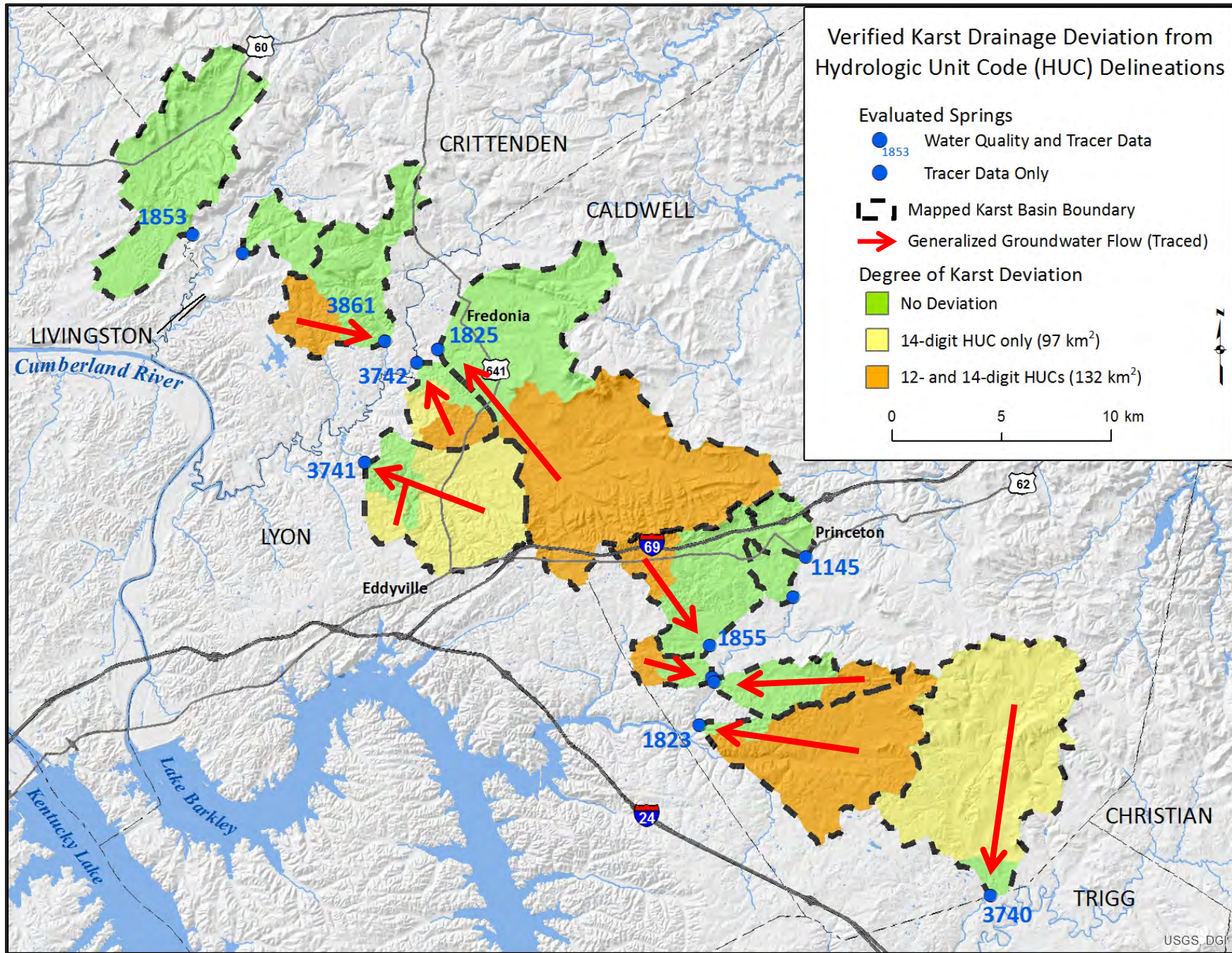
Figure 20. Verified Karst Drainage Deviation from HUC Boundaries
