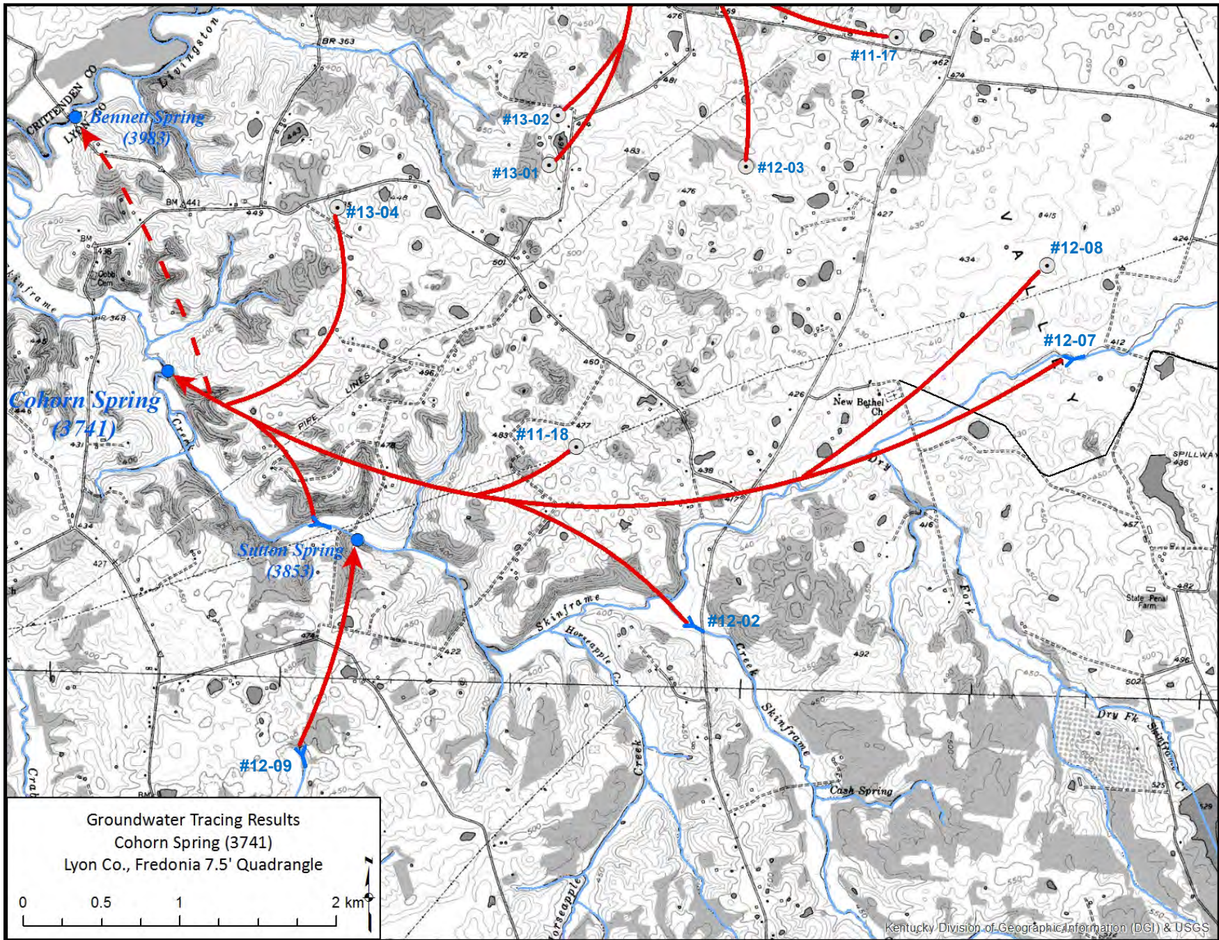
Figure 14. Cohorn Spring Tracer Map
