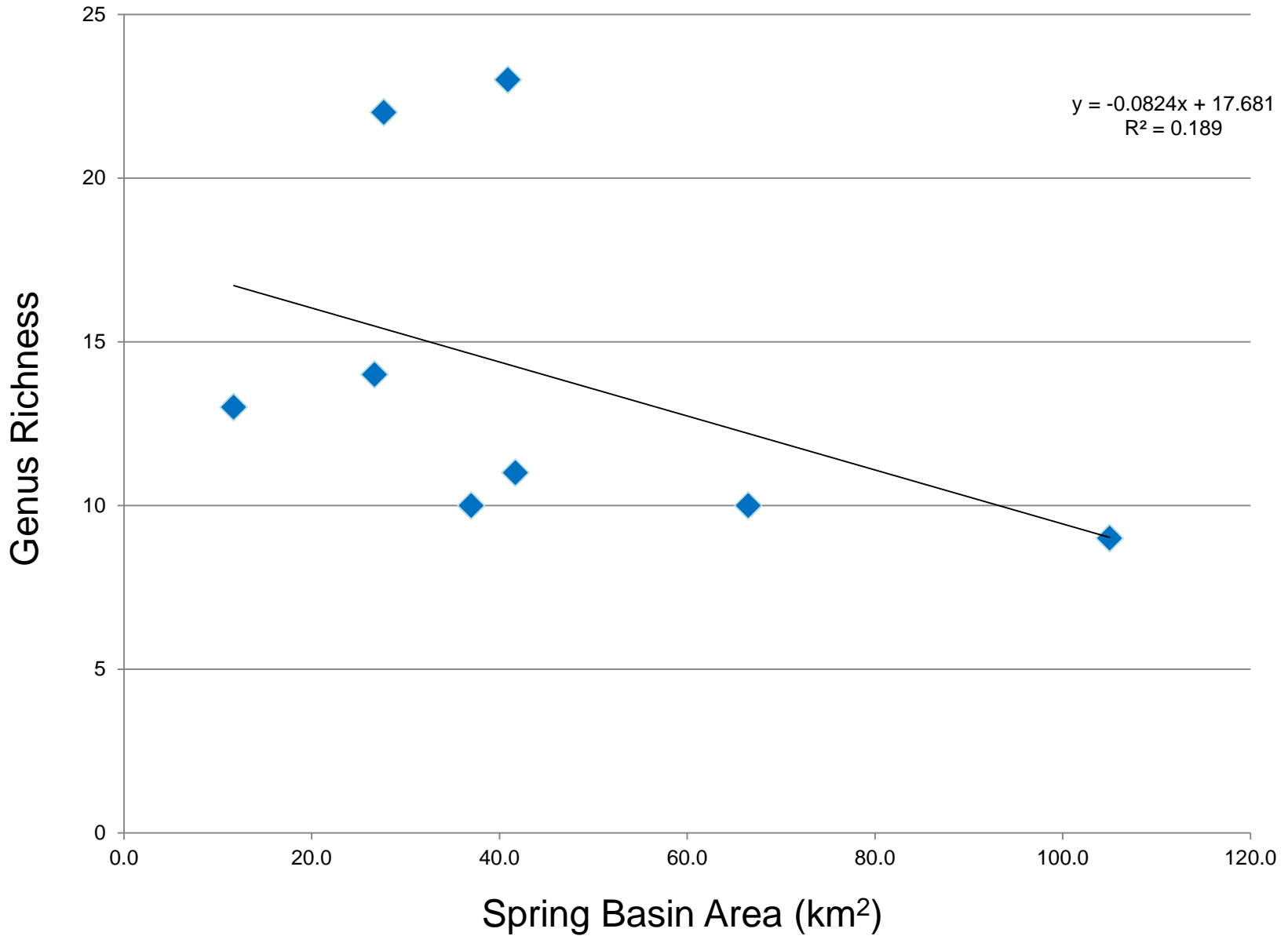
Figure 35. Relationship of Spring Basin Area to Taxa Richness
