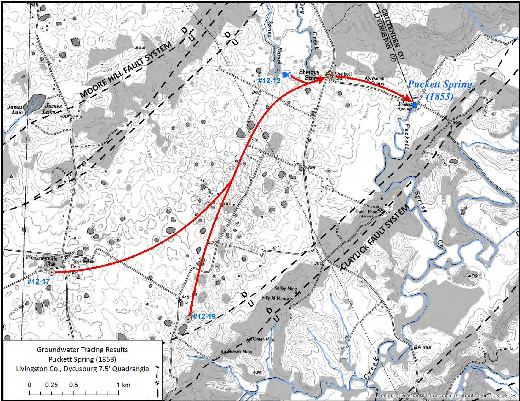
Figure 19. Puckett Spring Tracer Map
