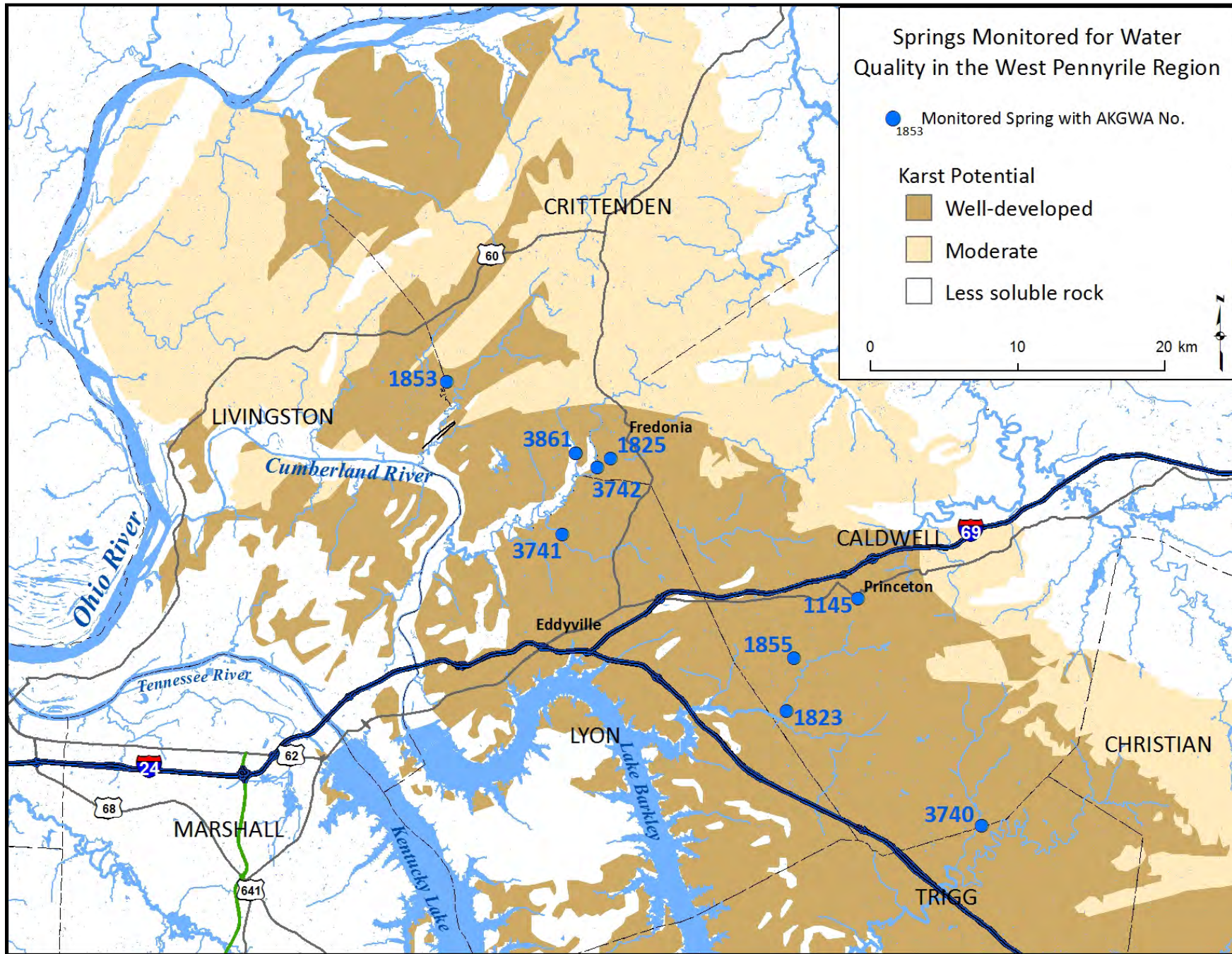
Figure 1. Map of Study Area Springs
