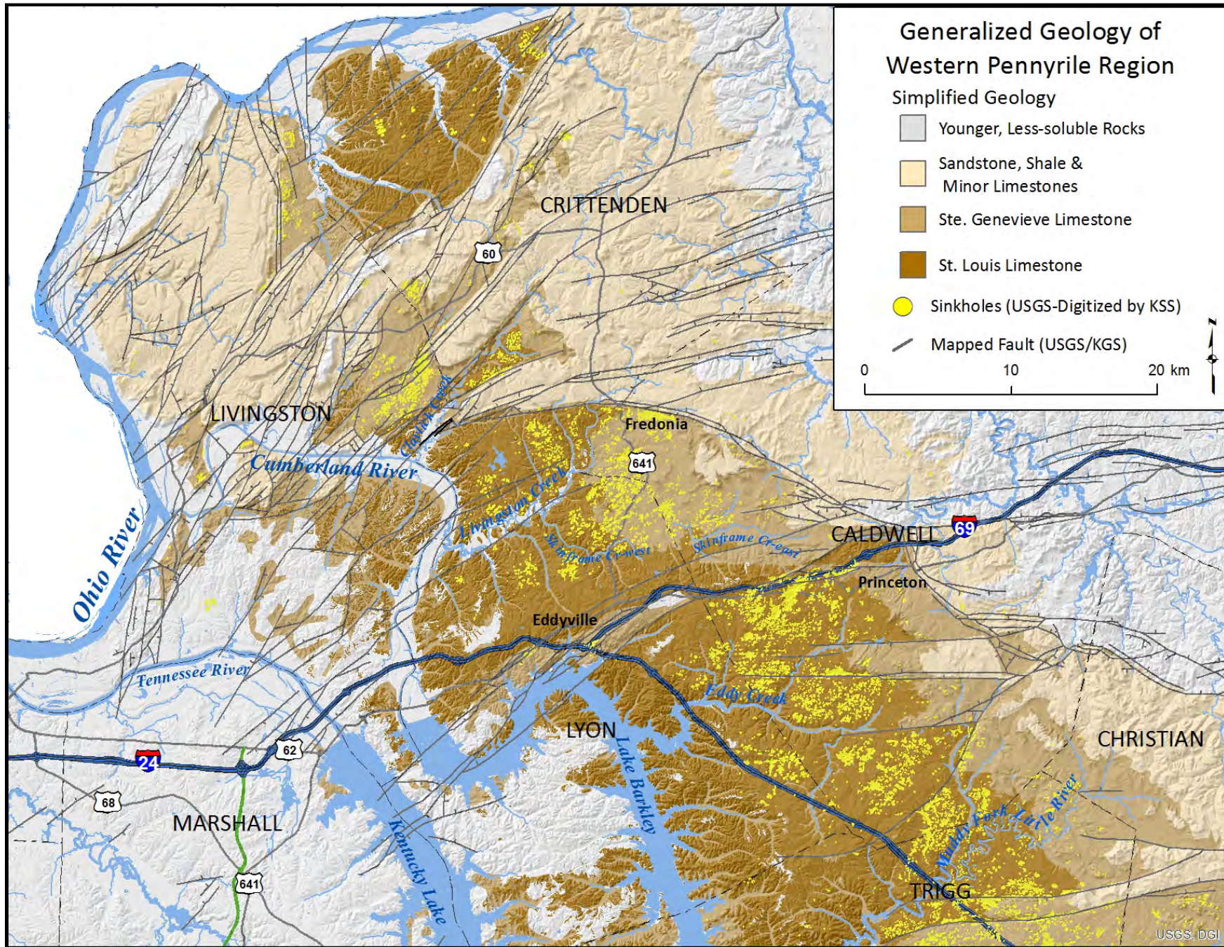
Figure 2. Hydrography and Geology of Lower Cumberland River in Kentucky
