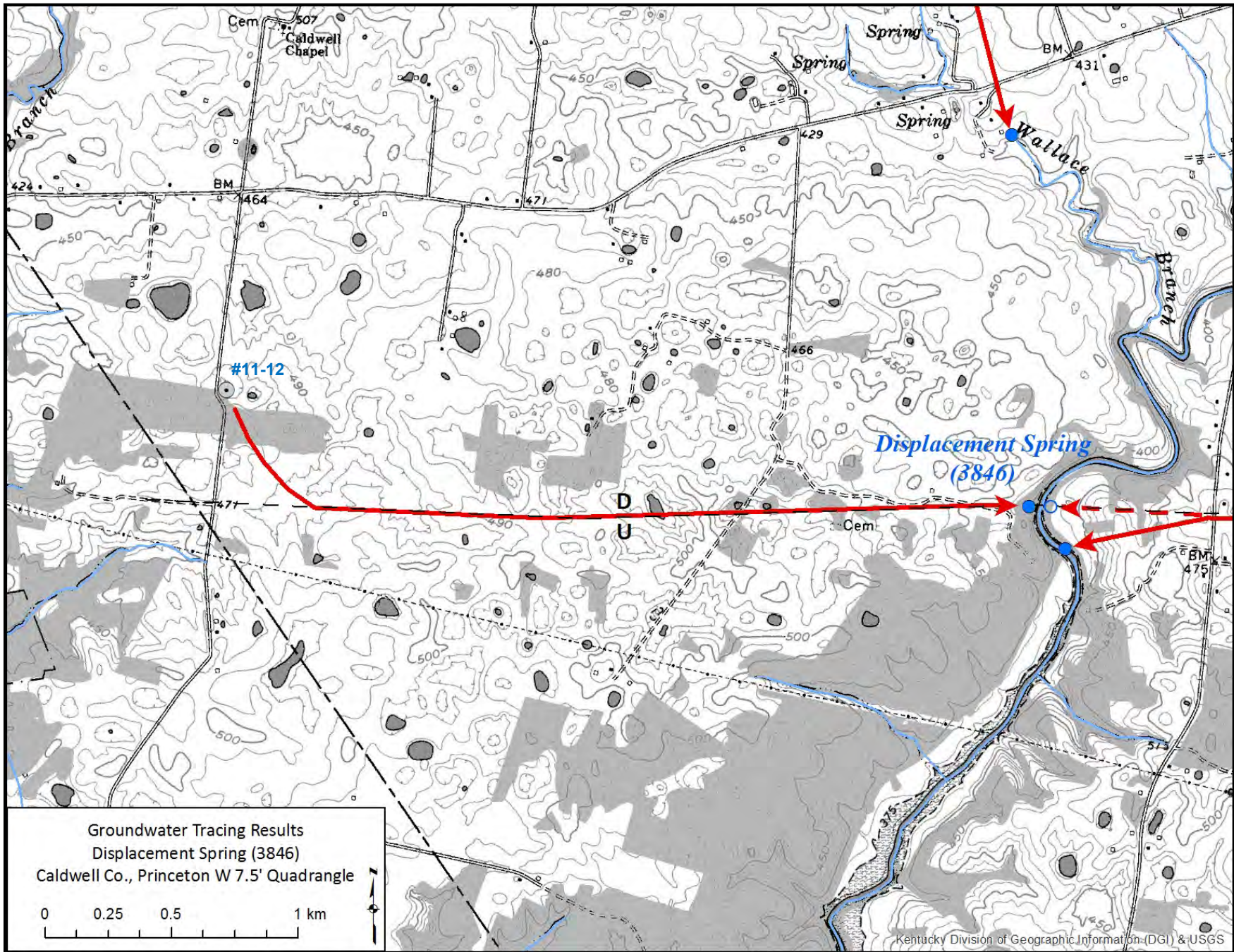
Figure 12. Displacement Spring Tracer Map
