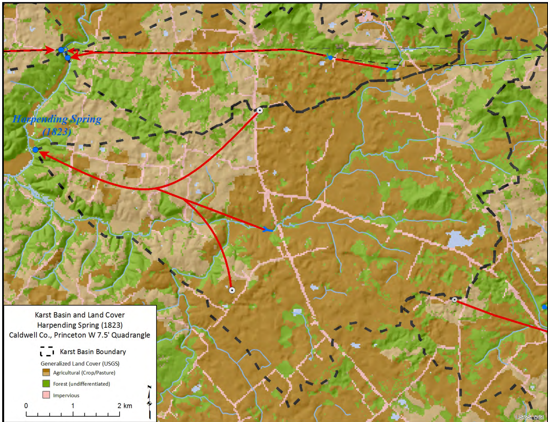
Figure 24. Harpending Spring Karst Basin and Land Cover Map (WAH-Full Support, PCR-Partial Support)
