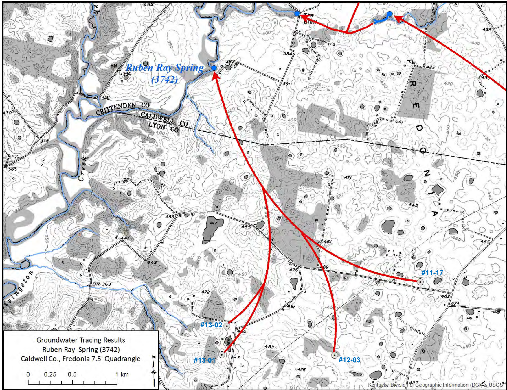
Figure 15. Ruben Ray Spring Tracer Map
