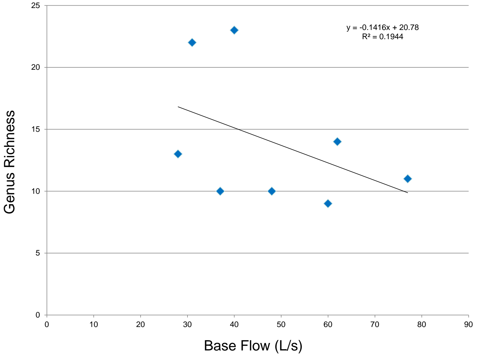
Figure 36. Relationship of Base Flow to Taxa Richness
