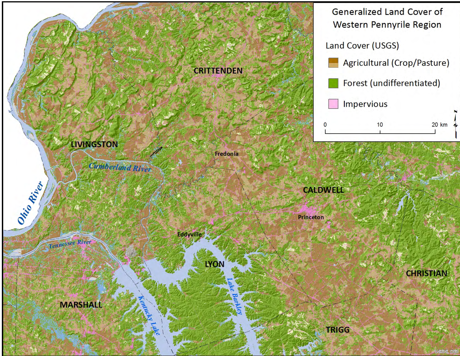
Figure 4. Generalized Land Cover of the West Pennyrile Region
