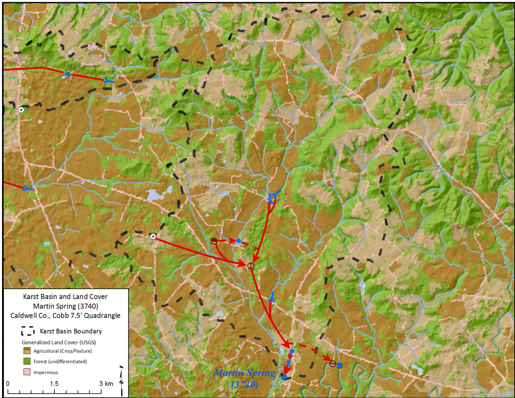
Figure 27. Martin Spring Karst Basin and Land Cover Map (WAH-Full Support, PCR-Partial Support)
