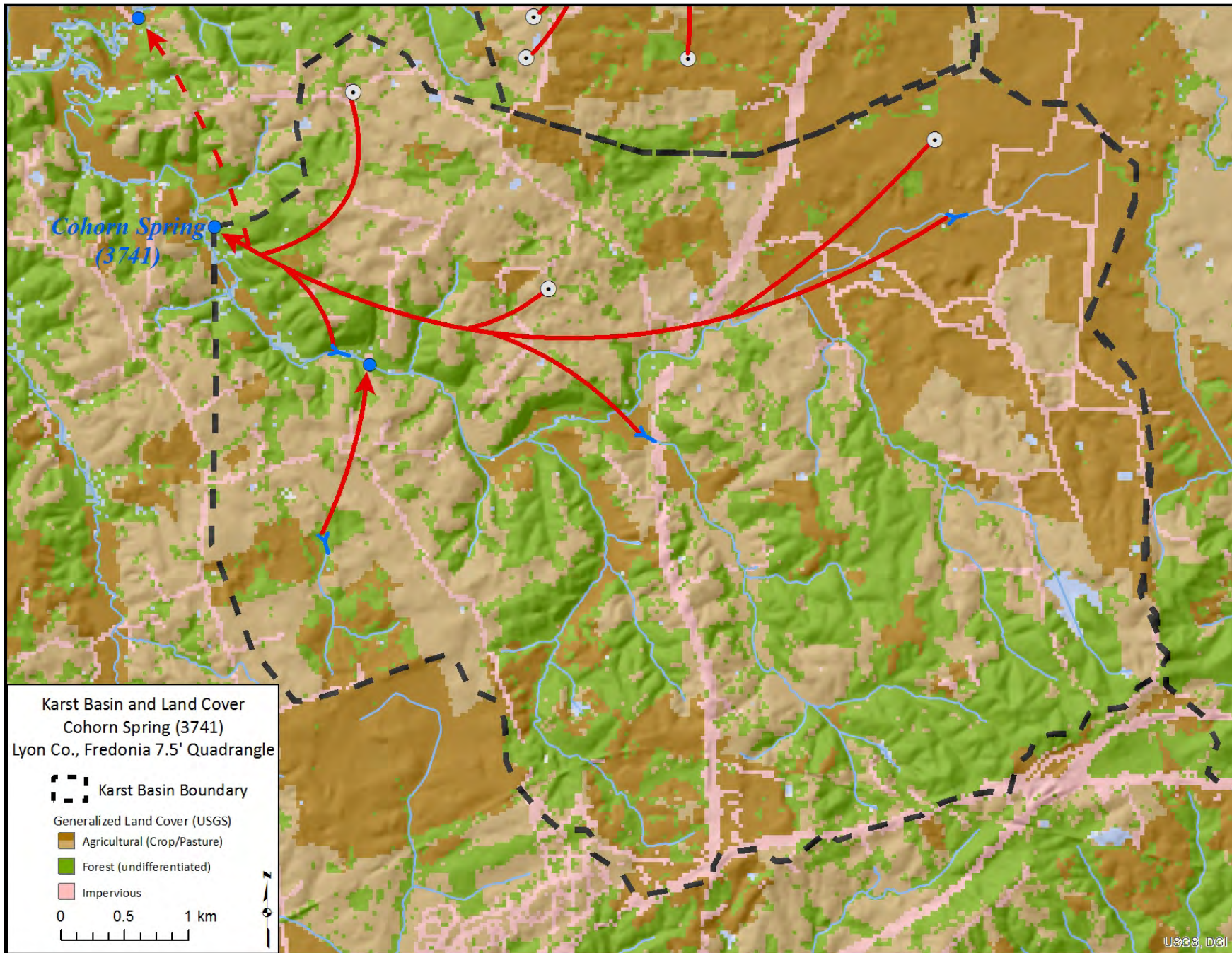
Figure 29. Cohorn Spring Karst Basin and Land Cover Map (WAH-Full Support, PCR-Full Support)
