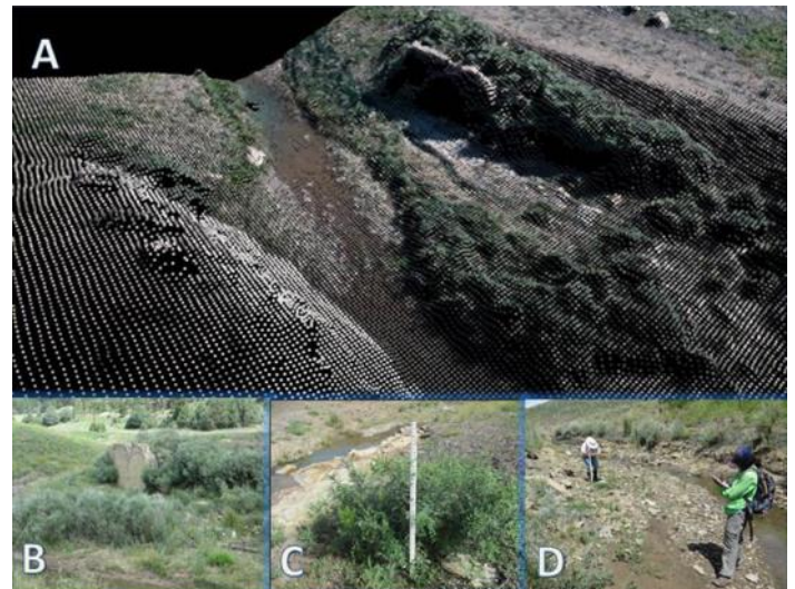
Figure 3. A) Point cloud of XYZ locations and RGB imagery values of a section of the stream in Dillon Canyon. A 3D representation view in Global Mapper vers. 15.2. B) Photo on the ground of the same section with closeup of willows (5-10 feet tall) and archaeological structures. C) Data validation samples included measures of vegetation species, height, diameter, and GPS location. D) Stream cross-section measurements were taken for a comparison to topographic surface model.
