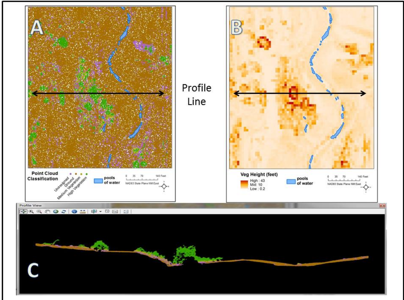
Figure 4. Canopy height analysis using ArcGIS 10.2.1 LiDAR tools. A) The point cloud was initially classified into ground, unassigned, medium and high vegetation. B) A vegetation height map was created by subtracting a digital elevation model based on ground points from a digital surface model based on all points that included vegetation. C) An elevation profile view created in ArcMap based on the point cloud classification.
